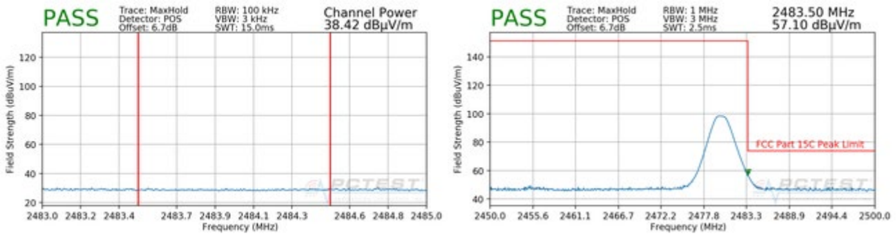
Plot 7-1. Radiated Restricted Upper Band Edge Measurement (Average & Peak)
