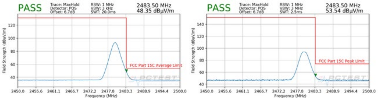
Plot 7-2. Radiated Restricted Upper Band Edge Measurement with WCP (Average & Peak)
