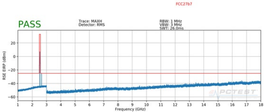
Plot 7-7. Radiated Spurious Plot 1GHz - 18GHz (Band 7)
