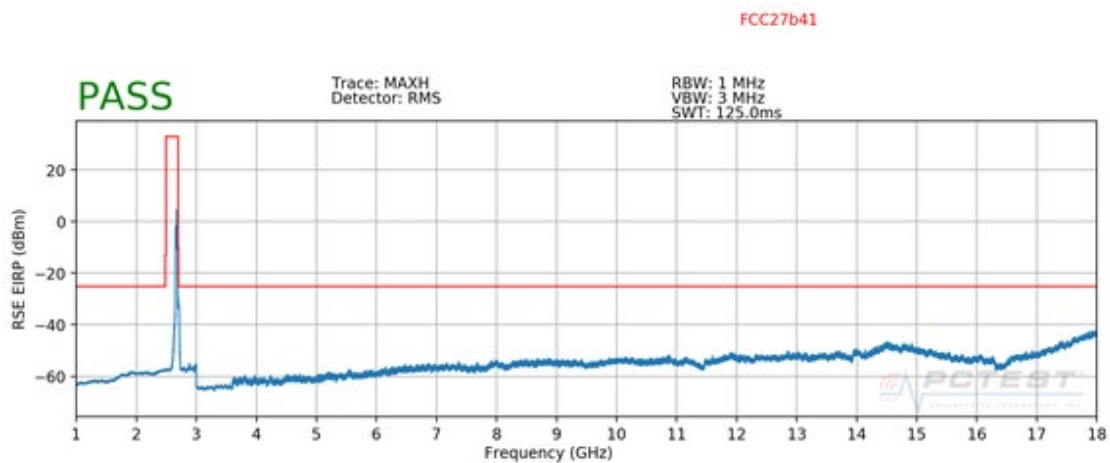
Plot 7-50. Radiated Spurious Plot (ULCA B41 - 20+20MHz - PCC: RB 100 Offset 0, SCC: RB 100 Offset 0 – High Channel)
