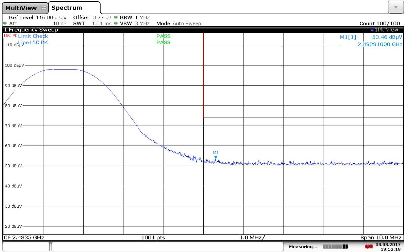
Plot 7-4. Radiated Restricted Upper Band Edge Measurement with WCP (Peak)
