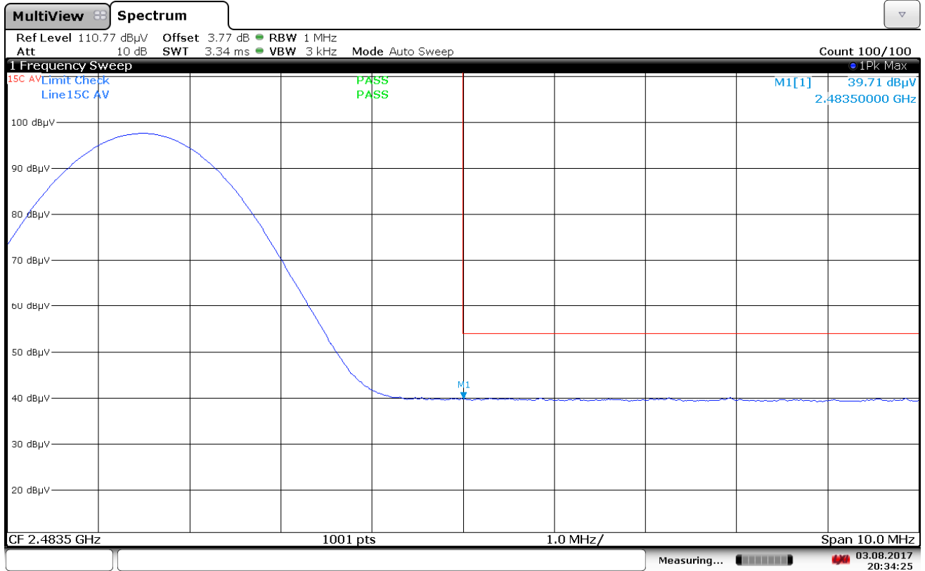
Plot 7-3. Radiated Restricted Upper Band Edge Measurement with WCP (Average)
