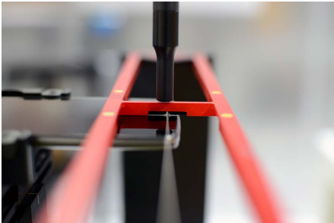
Figure 18-4 HAC Phantom Plane Alignment (Standard Battery Cover)
