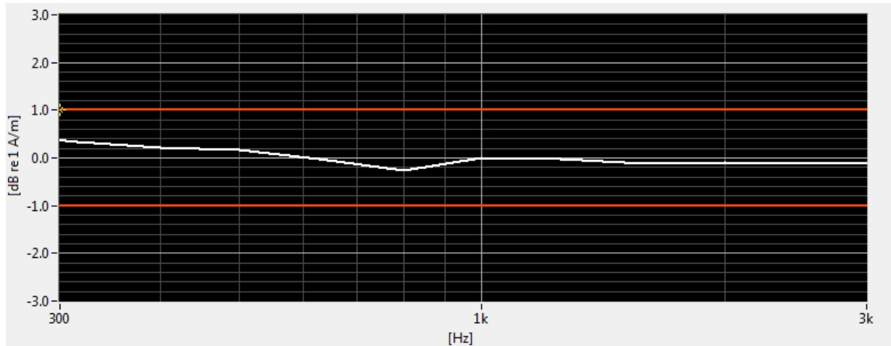
Figure 7-3 Helmholtz Coil Validation for Frequency Response
