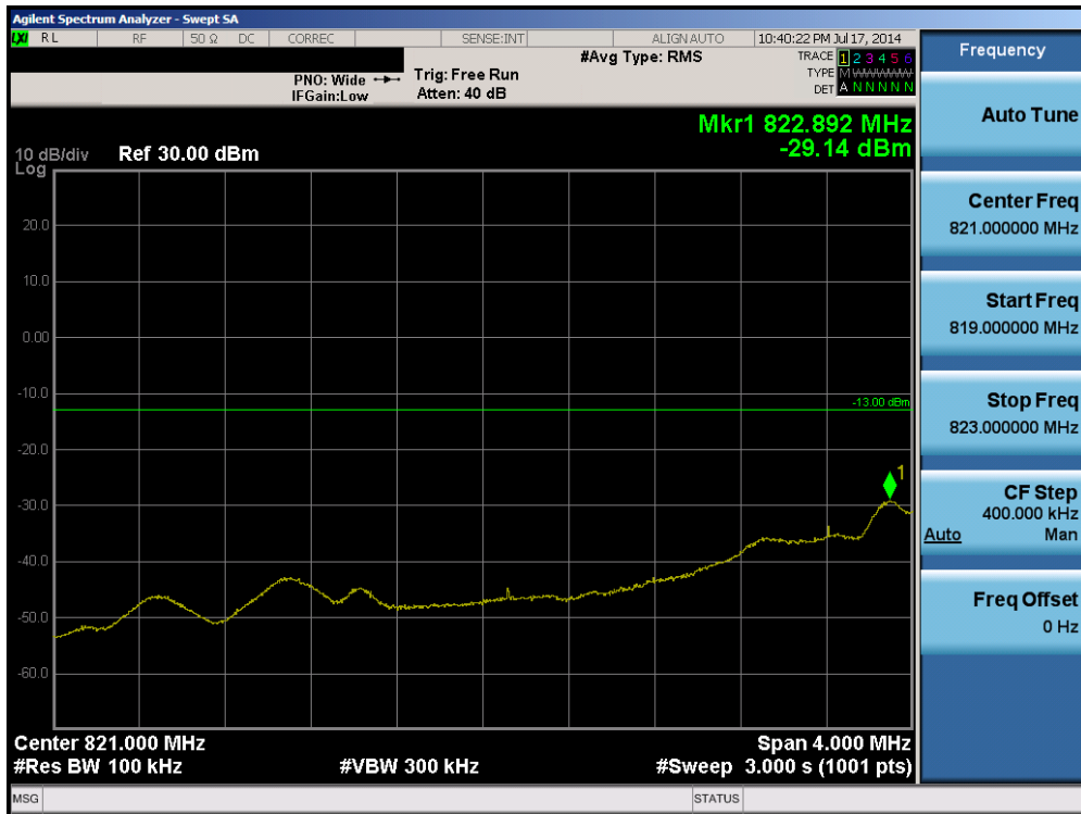
Plot 6-16. Band Edge Plot (Cellular CDMA Mode – Ch. 1013)
