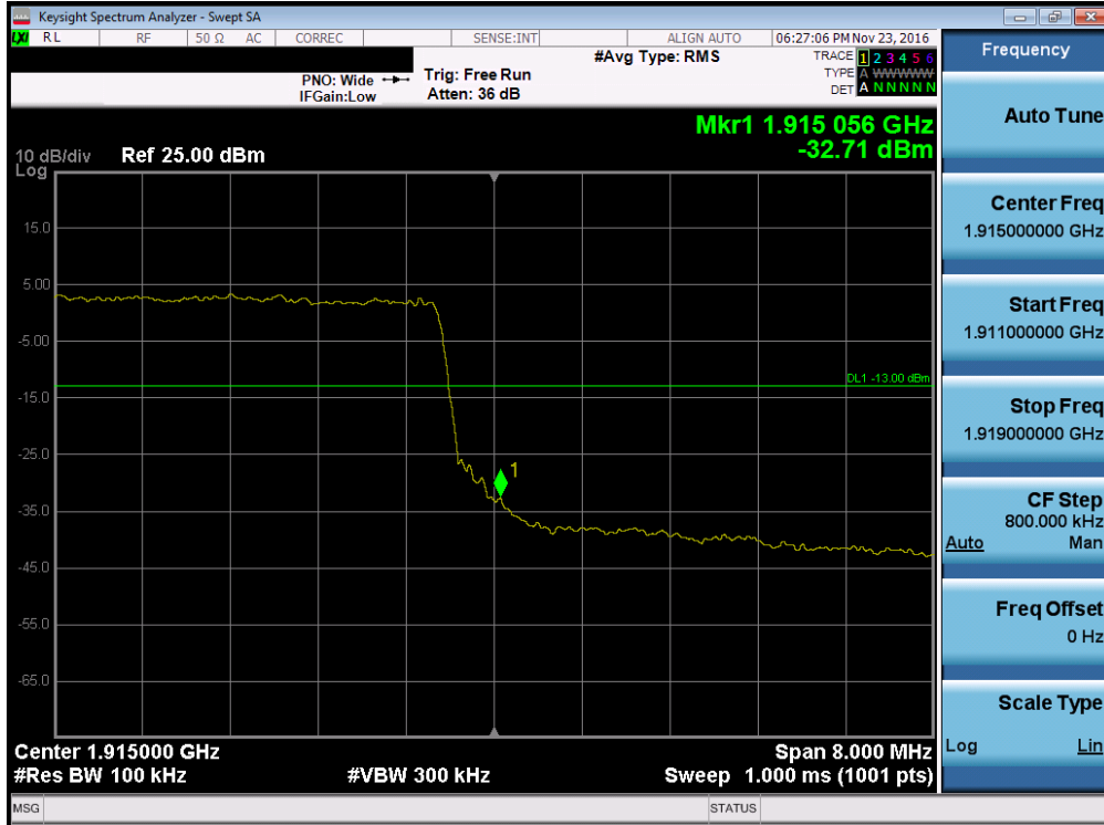
Plot 7-143. Upper Band Edge Plot (Band 2/25 – 10.0MHz QPSK – RB Size 50)
