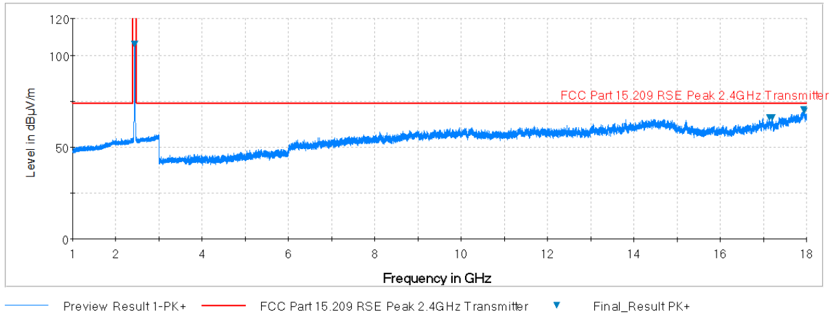
Plot 7-36. Radiated Spurious Plot above 1GHz (802.11b – Ch. 6, Ant. Pol. V)
