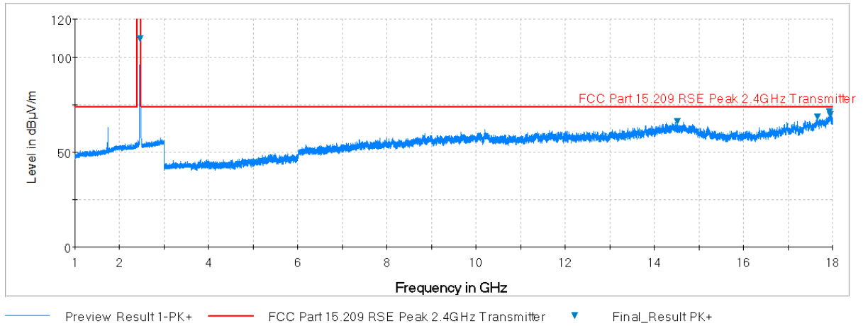
Plot 7-37. Radiated Spurious Plot above 1GHz (802.11b – Ch. 11, Ant. Pol. H)
