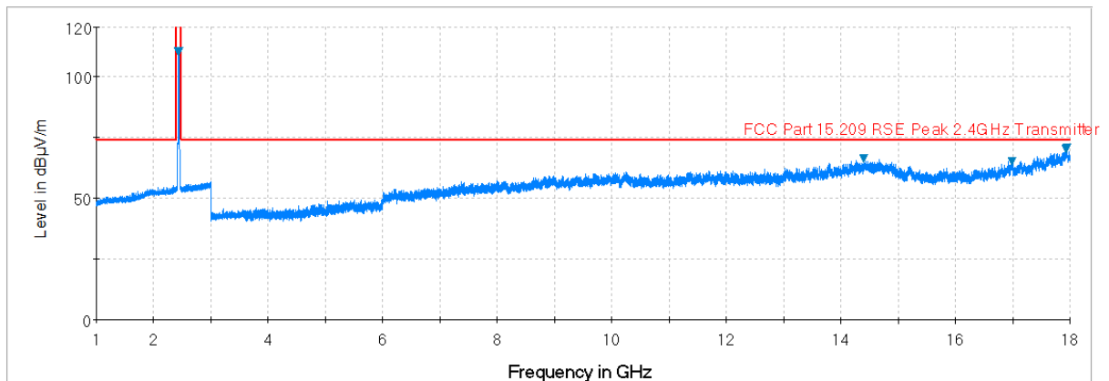
Preview Result 1-PK+ FCC Part 15.209 RSE Peak 2.4GHz Transmitter Final_Result PK+
