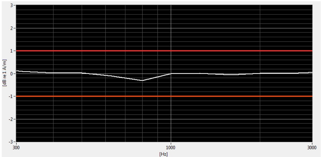
Figure 6-3 Helmholtz Coil Validation for Frequency Response
