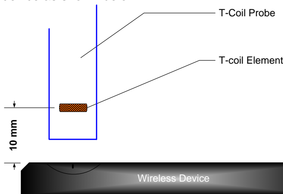
Figure 5-11 Measurement Distance
