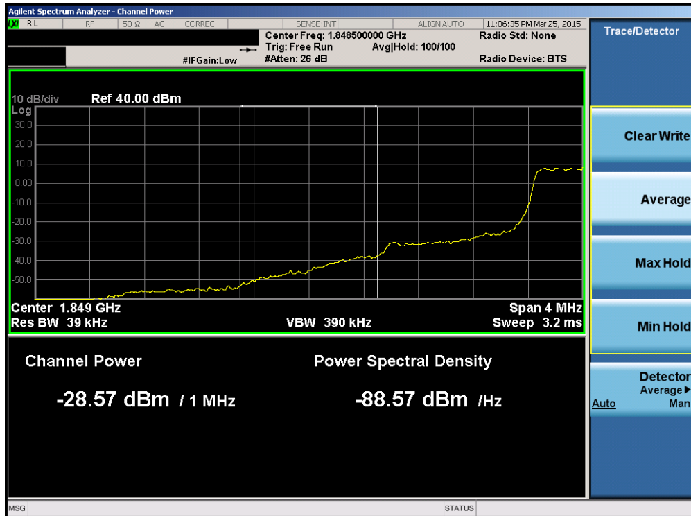
Plot 6-149. Lower Extended Band Edge Plot (Band 25 – 1.4MHz QPSK – RB Size 6)
