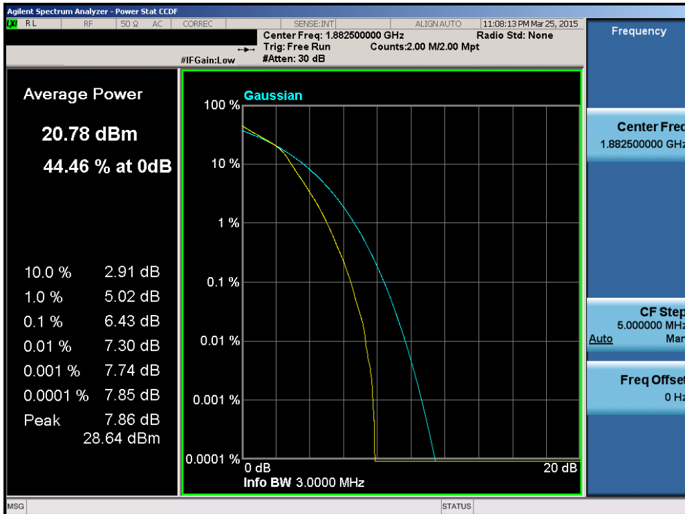
Plot 6-175. PAR Plot (Band 25 – 3.0MHz 16-QAM – RB Size 15)
