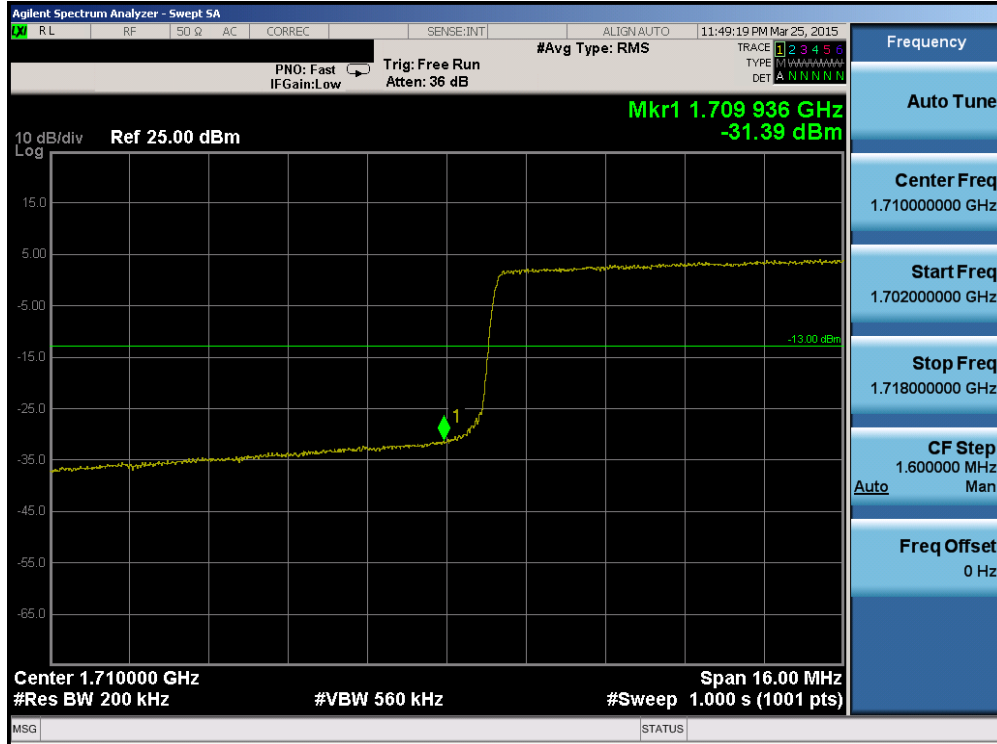
Plot 6-144. Lower Band Edge Plot (Band 4 – 20.0MHz QPSK – RB Size 100)
