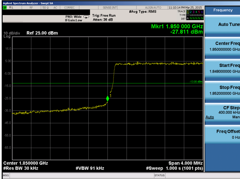
Plot 6-152. Lower Band Edge Plot (Band 25 – 3.0MHz QPSK – RB Size 15)
