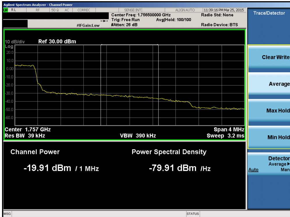
Plot 6-131. Upper Extended Band Edge Plot (Band 4 – 3.0MHz QPSK – RB Size 15)
