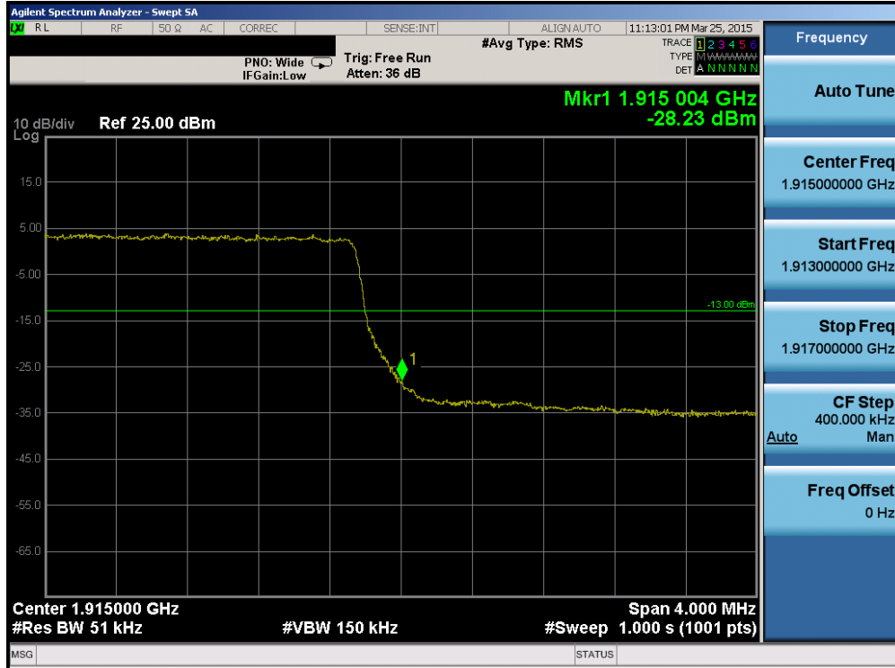
Plot 6-158. Upper Band Edge Plot (Band 25 – 5.0MHz QPSK – RB Size 25)
