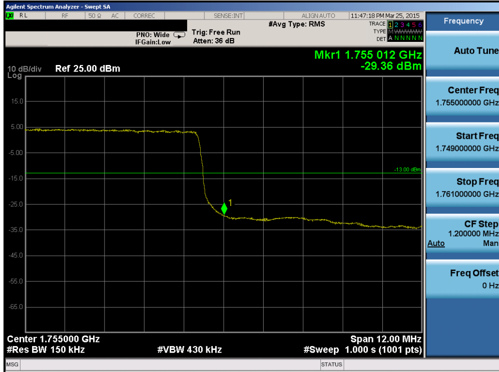
Plot 6-142. Upper Band Edge Plot (Band 4 – 15.0MHz QPSK – RB Size 75)
