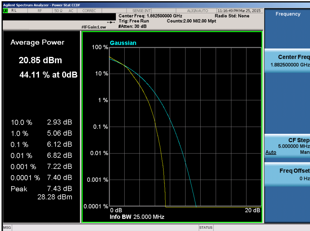
Plot 6-181. PAR Plot (Band 25 – 15.0MHz 16-QAM – RB Size 75)
