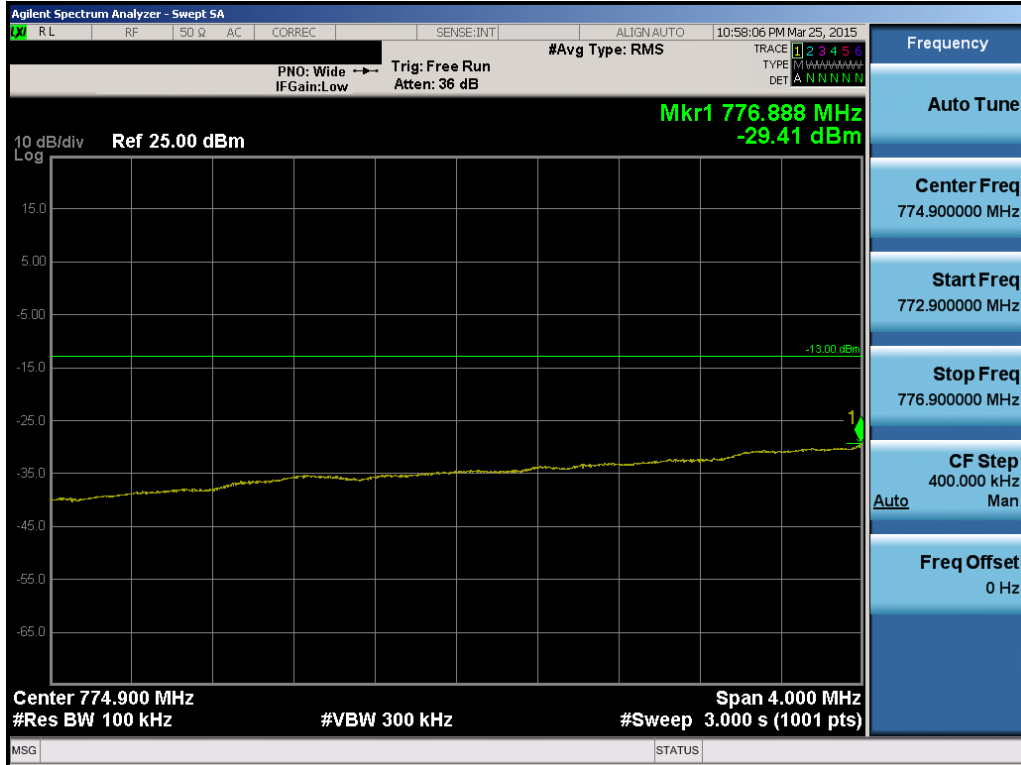
Plot 6-100. Lower Extended Band Edge Plot (Band 13 – 5.0MHz QPSK – RB Size 25)
