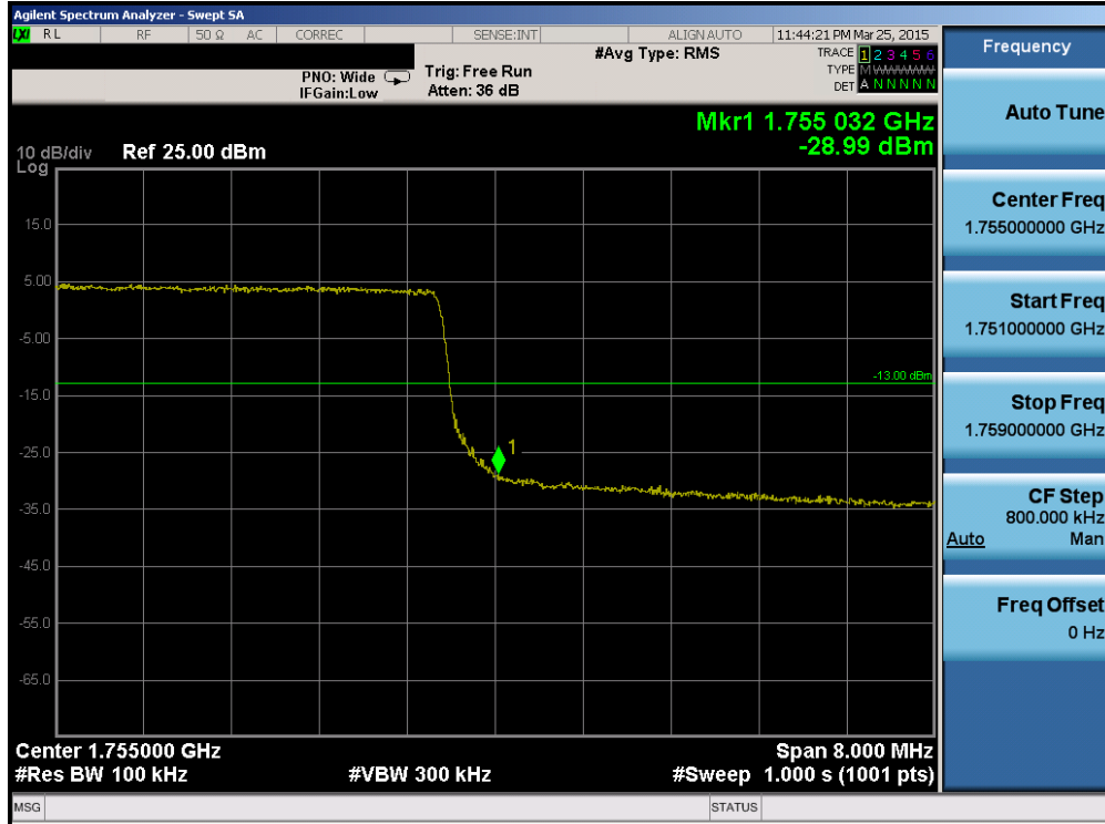
Plot 6-138. Upper Band Edge Plot (Band 4 – 10.0MHz QPSK – RB Size 50)
