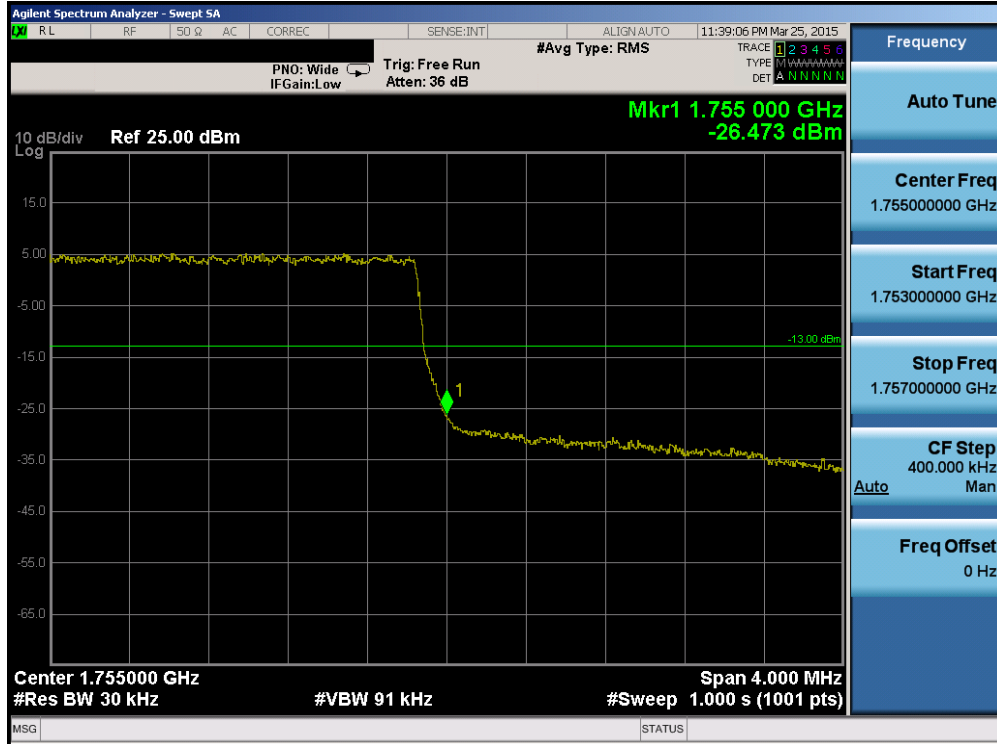
Plot 6-130. Upper Band Edge Plot (Band 4 – 3.0MHz QPSK – RB Size 15)
