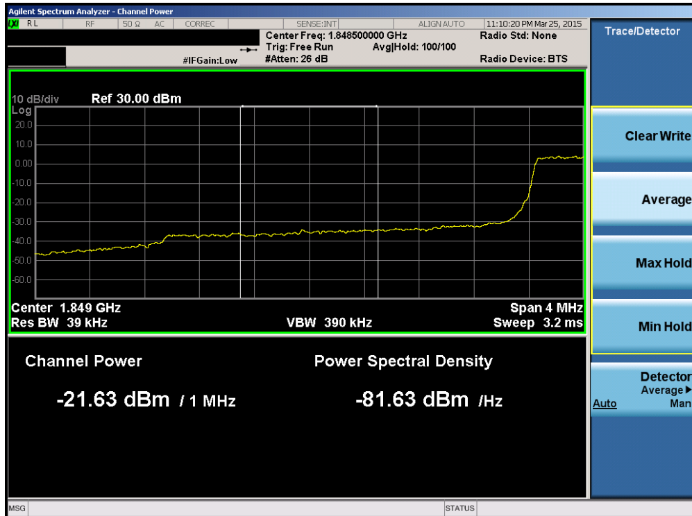
Plot 6-153. Lower Extended Band Edge Plot (Band 25 – 3.0MHz QPSK – RB Size 15)
