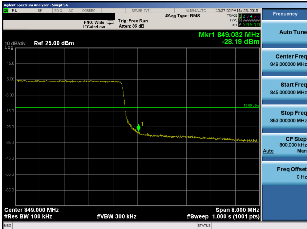
Plot 6-123. Upper Band Edge Plot (Band 5 – 10.0MHz QPSK – RB Size 50)
