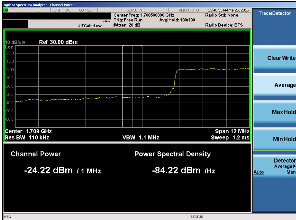
Plot 6-141. Lower Extended Band Edge Plot (Band 4 – 15.0MHz QPSK – RB Size 75)
