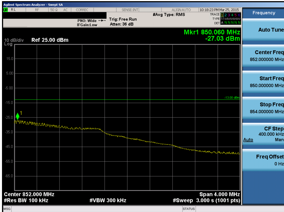
Plot 6-117. Upper Extended Band Edge Plot (Band 5 – Band 5 – 3.0MHz QPSK – RB Size 15)
