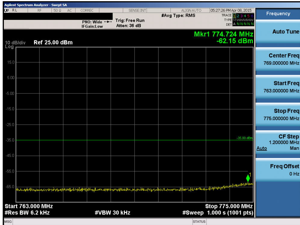
Plot 6-105. Lower Emission Mask Edge Plot (Band 13 – 10.0MHz QPSK – RB Size 50)
