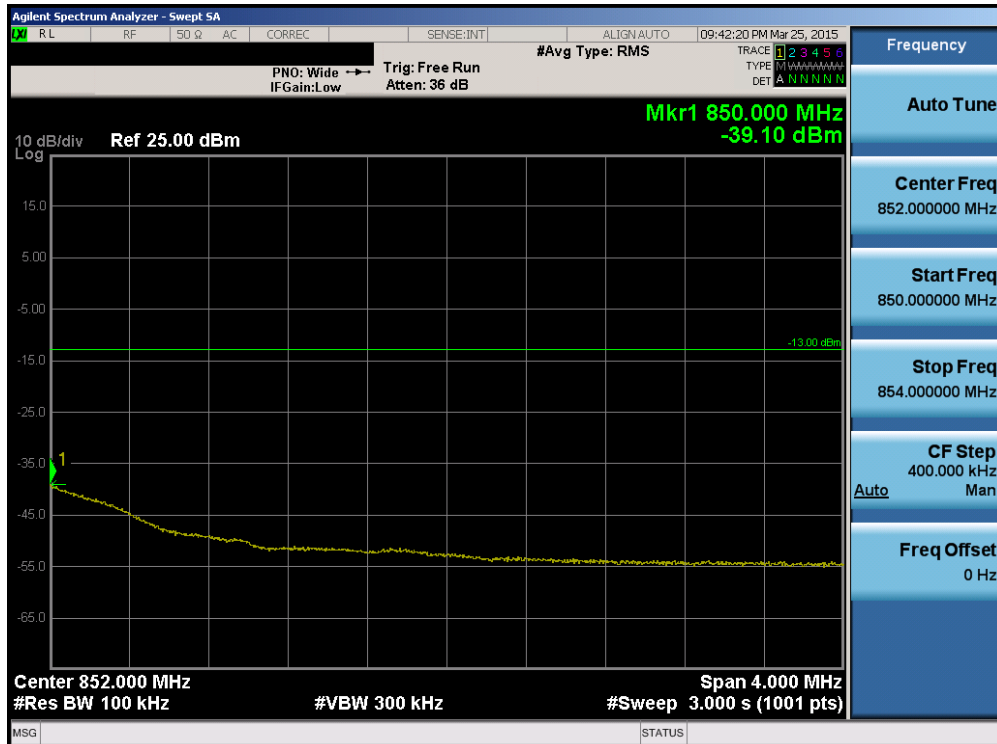
Plot 6-113. Upper Extended Band Edge Plot (Band 5 – 1.4MHz QPSK – RB Size 6)
