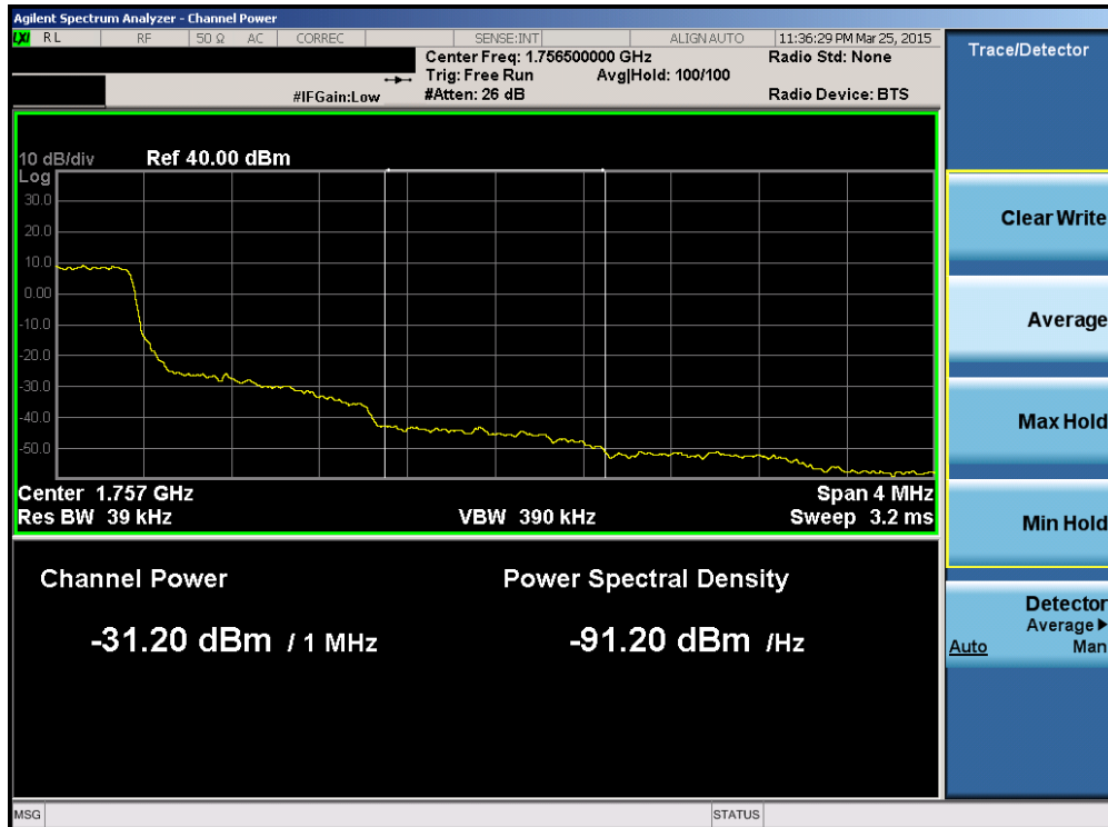
Plot 6-127. Upper Extended Band Edge Plot (Band 4 – 1.4MHz QPSK – RB Size 6)
