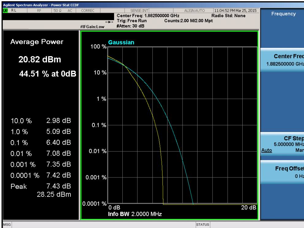
Plot 6-173. PAR Plot (Band 25 – 1.4MHz 16-QAM – RB Size 6)
