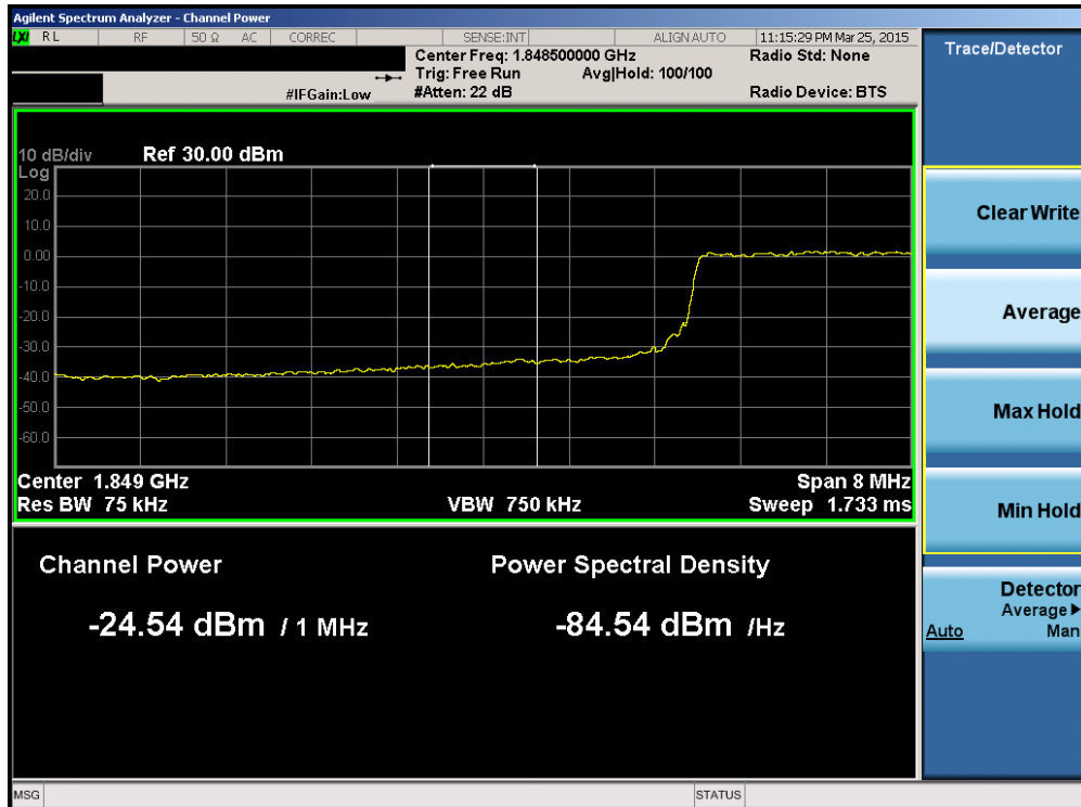
Plot 6-161. Lower Extended Band Edge Plot (Band 25 – 10.0MHz QPSK – RB Size 50)
