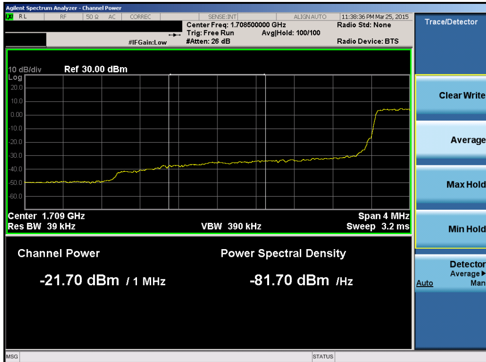
Plot 6-129. Lower Extended Band Edge Plot (Band 4 – 3.0MHz QPSK – RB Size 15)
