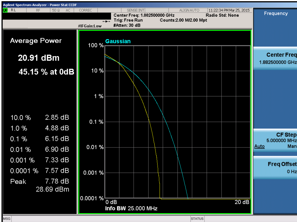
Plot 6-183. PAR Plot (Band 25 – 20.0MHz 16-QAM – RB Size 100)
