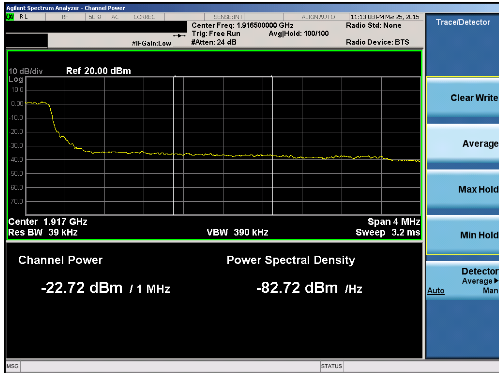
Plot 6-159. Upper Extended Band Edge Plot (Band 25 – 5.0MHz QPSK – RB Size 25)
