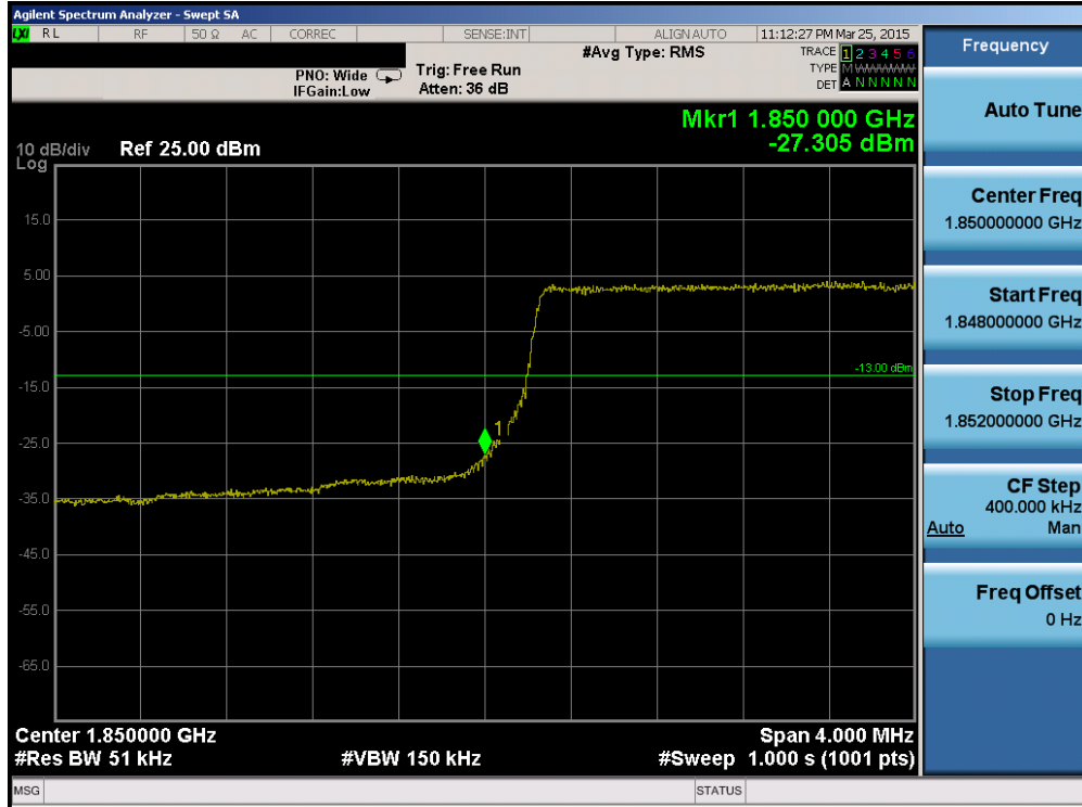
Plot 6-156. Lower Band Edge Plot (Band 25 – 5.0MHz QPSK – RB Size 25)
