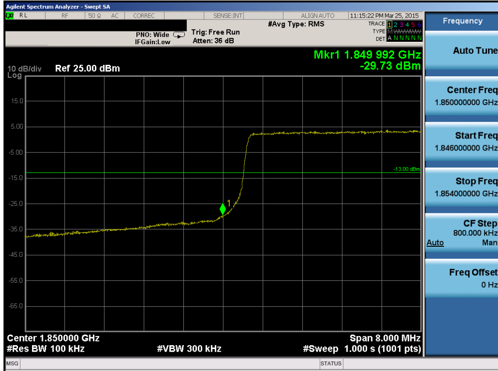
Plot 6-160. Lower Band Edge Plot (Band 25 – 10.0MHz QPSK – RB Size 50)
