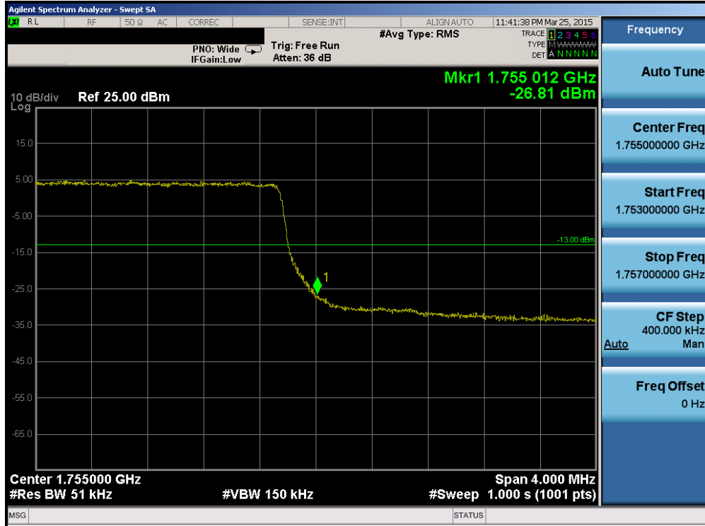
Plot 6-134. Upper Band Edge Plot (Band 4 – 5.0MHz QPSK – RB Size 25)
