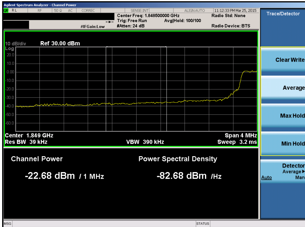
Plot 6-157. Lower Extended Band Edge Plot (Band 25 – 5.0MHz QPSK – RB Size 25)
