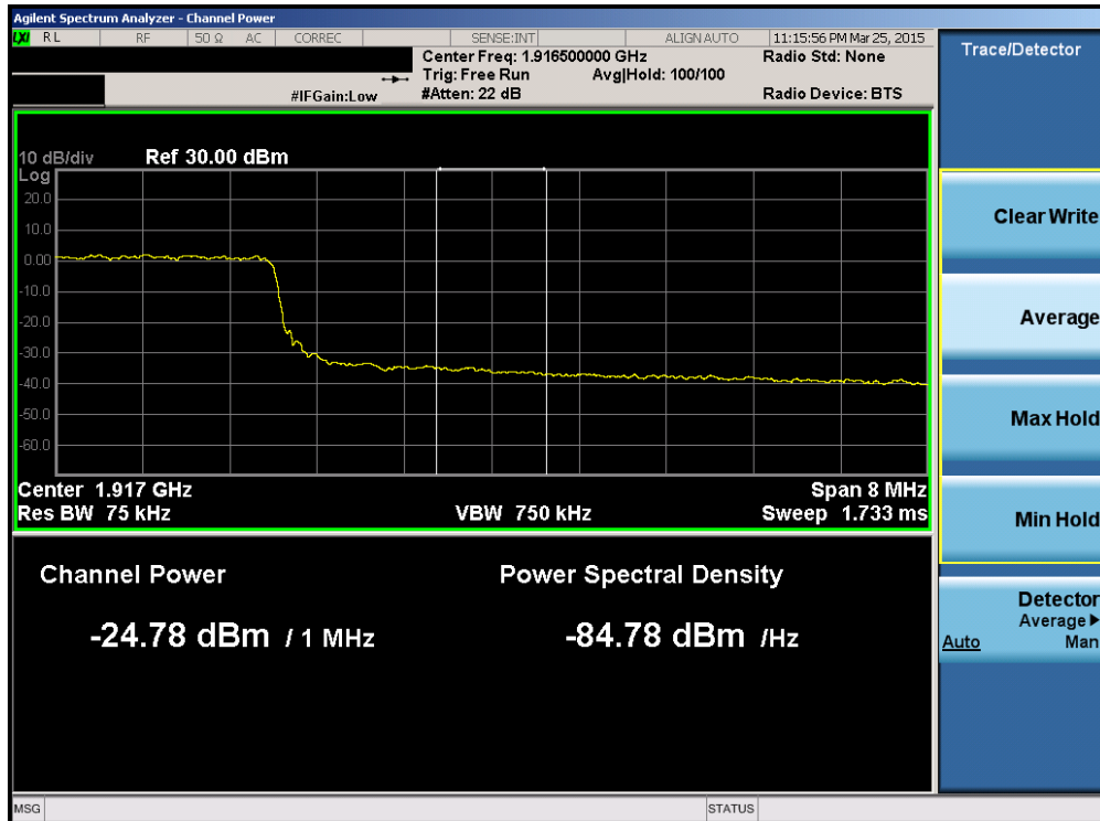
Plot 6-163. Upper Extended Band Edge Plot (Band 25 – 10.0MHz QPSK – RB Size 50)
