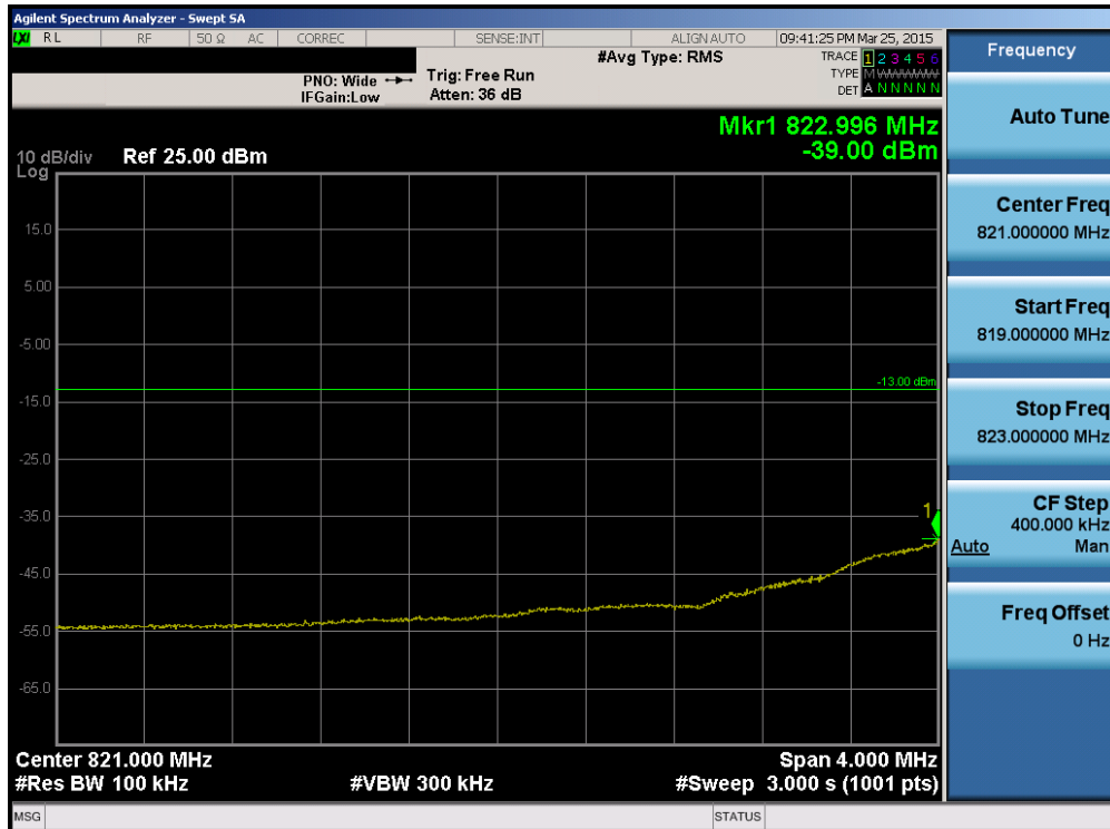
Plot 6-111. Lower Extended Band Edge Plot (Band 5 – 1.4MHz QPSK – RB Size 6)
