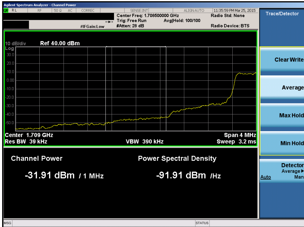
Plot 6-125. Lower Extended Band Edge Plot (Band 4 – 1.4MHz QPSK – RB Size 6)
