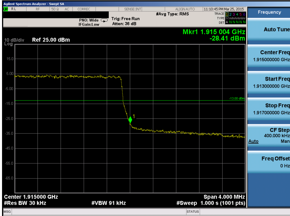
Plot 6-154. Upper Band Edge Plot (Band 25 – 3.0MHz QPSK – RB Size 15)
