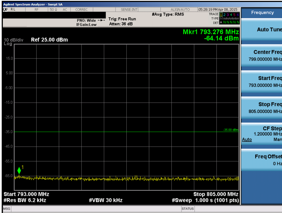
Plot 6-108. Upper Emission Mask Edge Plot (Band 13 – 10.0MHz QPSK – RB Size 50)
