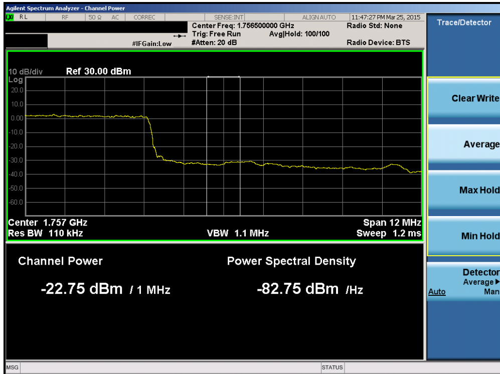
Plot 6-143. Upper Extended Band Edge Plot (Band 4 – 15.0MHz QPSK – RB Size 75)
