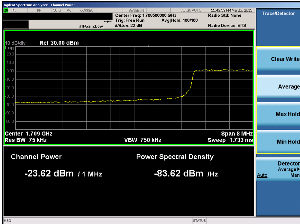
Plot 6-137. Lower Extended Band Edge Plot (Band 4 – 10.0MHz QPSK – RB Size 50)
