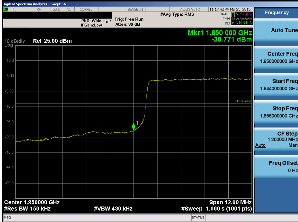
Plot 6-164. Lower Band Edge Plot (Band 25 – 15.0MHz QPSK – RB Size 75)
