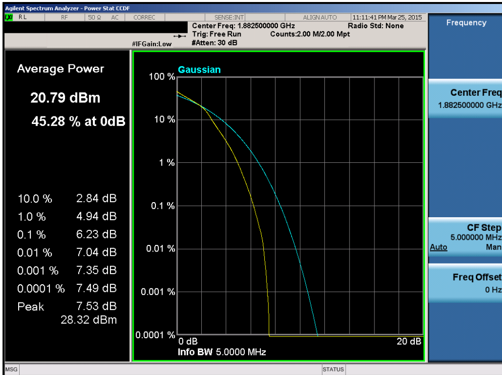
Plot 6-177. PAR Plot (Band 25 – 5.0MHz 16-QAM – RB Size 25)
