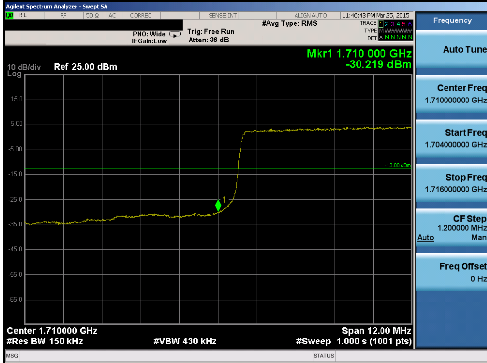
Plot 6-140. Lower Band Edge Plot (Band 4 – 15.0MHz QPSK – RB Size 75)
