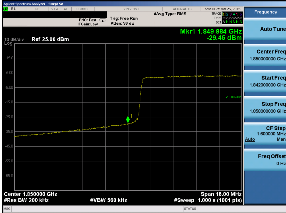
Plot 6-168. Lower Band Edge Plot (Band 25 – 20.0MHz QPSK – RB Size 100)
