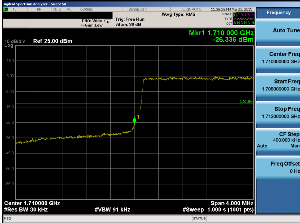
Plot 6-128. Lower Band Edge Plot (Band 4 – 3.0MHz QPSK – RB Size 15)
