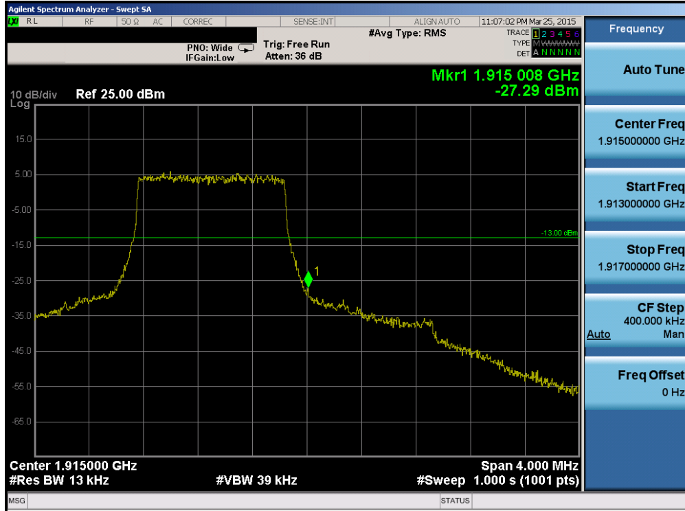
Plot 6-150. Upper Band Edge Plot (Band 25 – 1.4MHz QPSK – RB Size 6)
