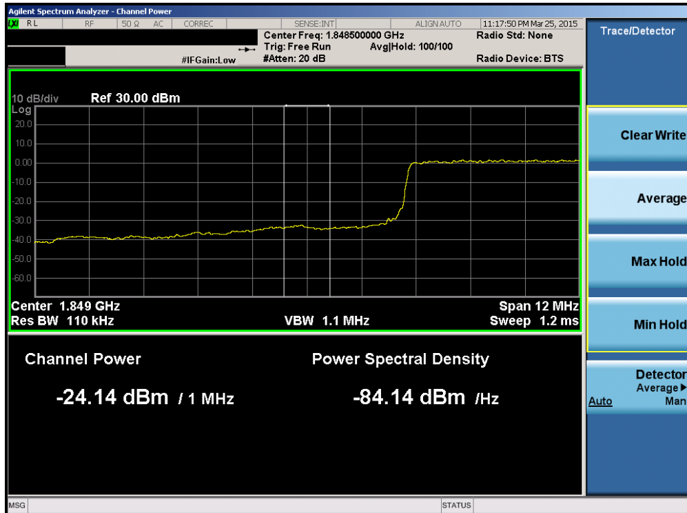
Plot 6-165. Lower Extended Band Edge Plot (Band 25 – 15.0MHz QPSK – RB Size 75)
