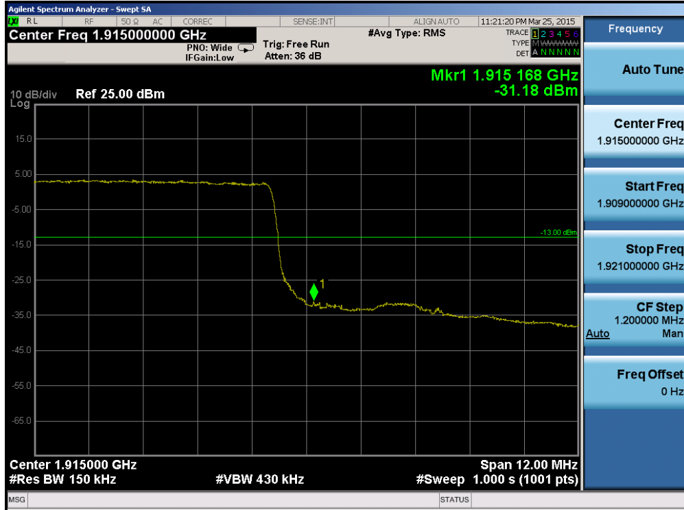
Plot 6-166. Upper Band Edge Plot (Band 25 – 15.0MHz QPSK – RB Size 75)
