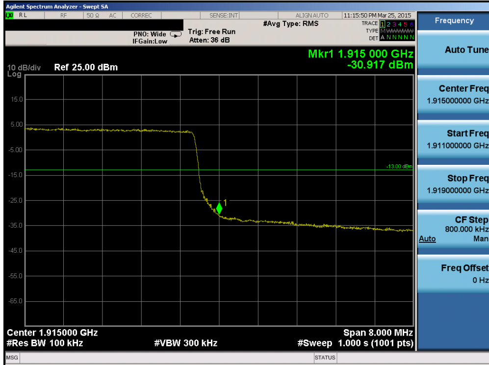
Plot 6-162. Upper Band Edge Plot (Band 25 – 10.0MHz QPSK – RB Size 50)
