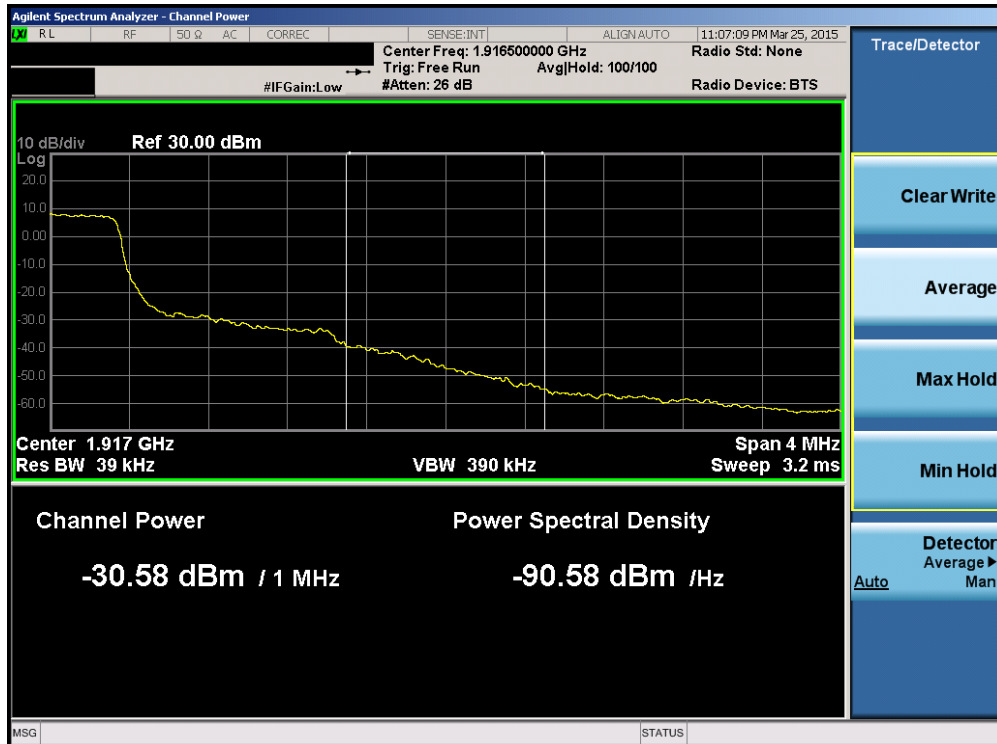
Plot 6-151. Upper Extended Band Edge Plot (Band 25 – 1.4MHz QPSK – RB Size 6)
