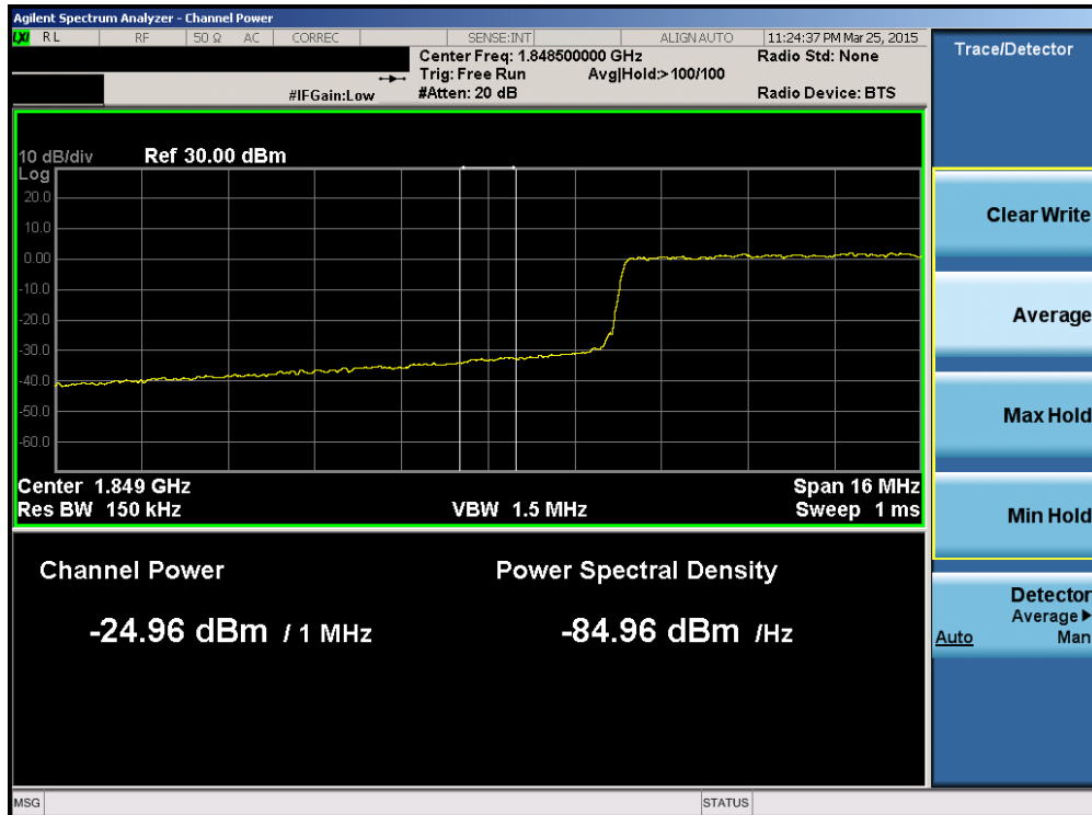
Plot 6-169. Lower Extended Band Edge Plot (Band 25 – 20.0MHz QPSK – RB Size 100)
