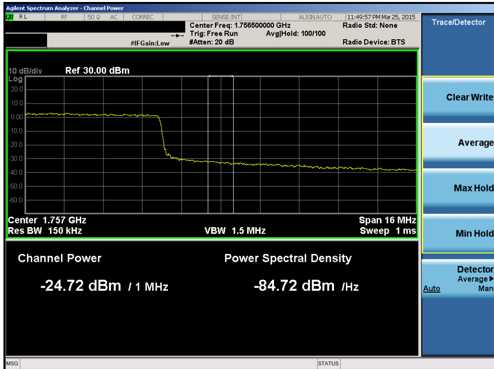
Plot 6-147. Upper Extended Band Edge Plot (Band 4 – 20.0MHz QPSK – RB Size 100)
