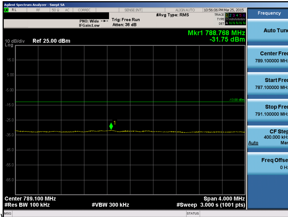
Plot 6-109. Upper Extended Band Edge Plot (Band 13 – 10.0MHz QPSK – RB Size 50)
