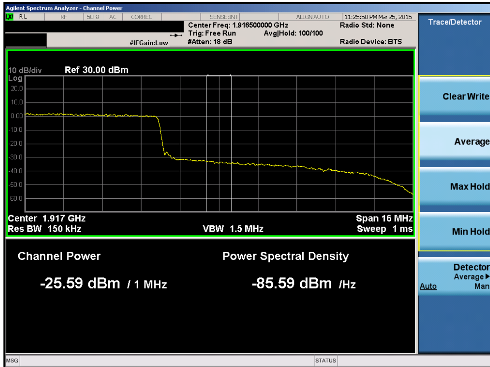
Plot 6-171. Upper Extended Band Edge Plot (Band 25 – 20.0MHz QPSK – RB Size 100)
