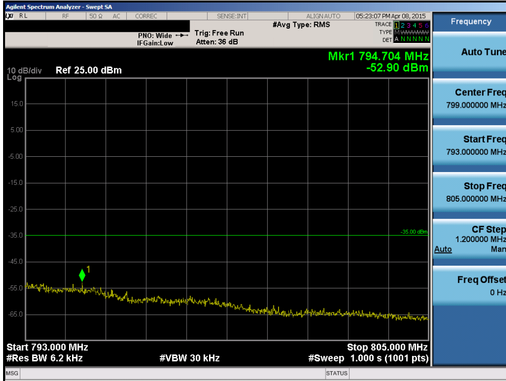
Plot 6-102. Upper Emission Mask Edge Plot (Band 13 – 5.0MHz QPSK – RB Size 25)
