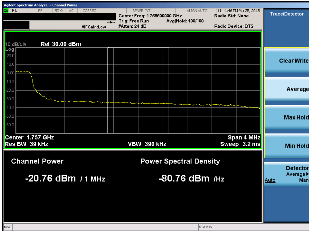
Plot 6-135. Upper Extended Band Edge Plot (Band 4 – 5.0MHz QPSK – RB Size 25)
