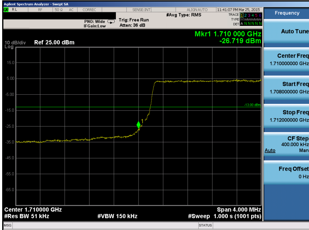
Plot 6-132. Lower Band Edge Plot (Band 4 – 5.0MHz QPSK – RB Size 25)
