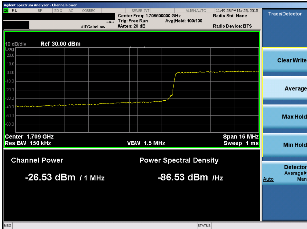
Plot 6-145. Lower Extended Band Edge Plot (Band 4 – 20.0MHz QPSK – RB Size 100)
