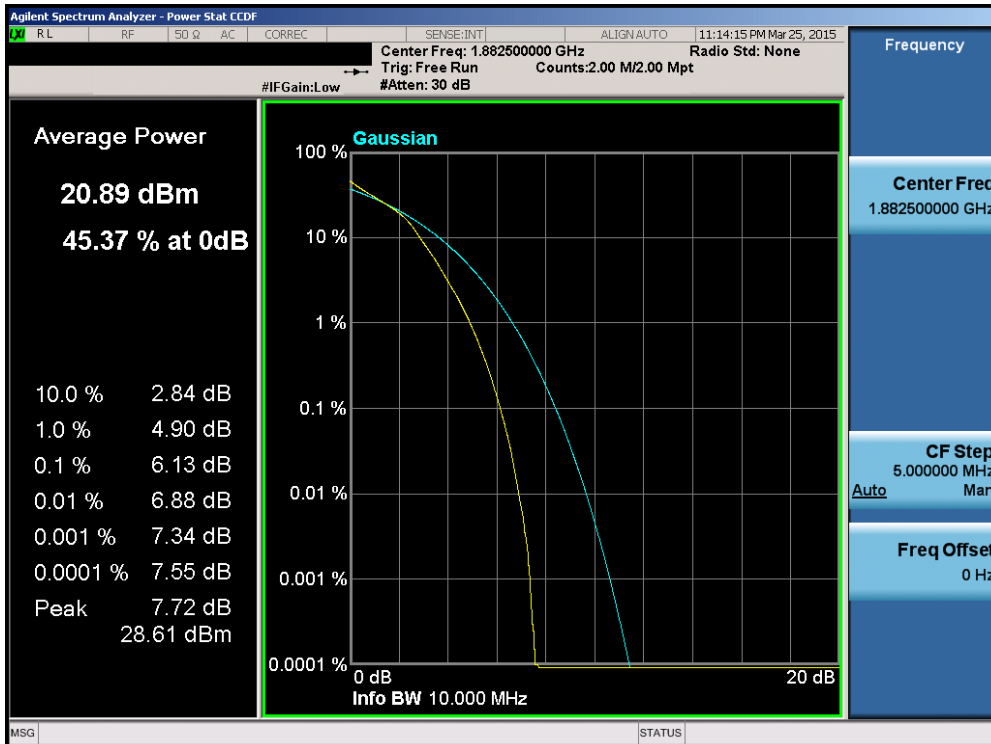
Plot 6-179. PAR Plot (Band 25 – 10.0MHz 16-QAM – RB Size 50)
