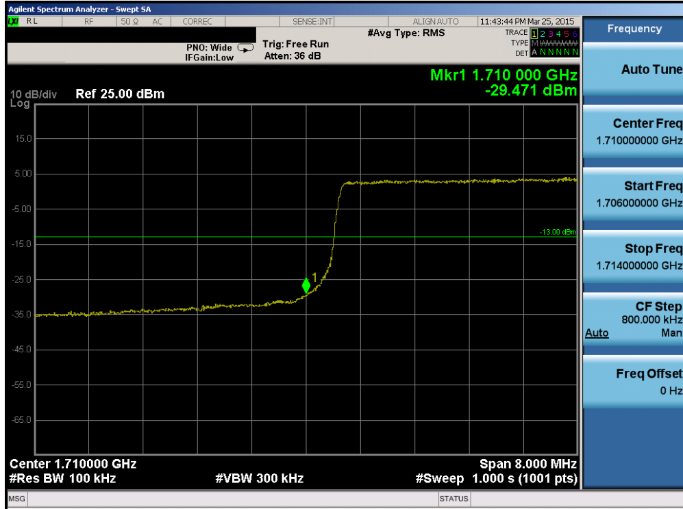
Plot 6-136. Lower Band Edge Plot (Band 4 – 10.0MHz QPSK – RB Size 50)
