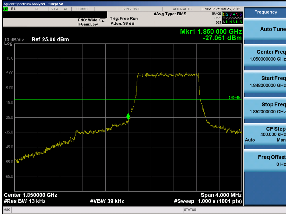
Plot 6-148. Lower Band Edge Plot (Band 25 – 1.4MHz QPSK – RB Size 6)
