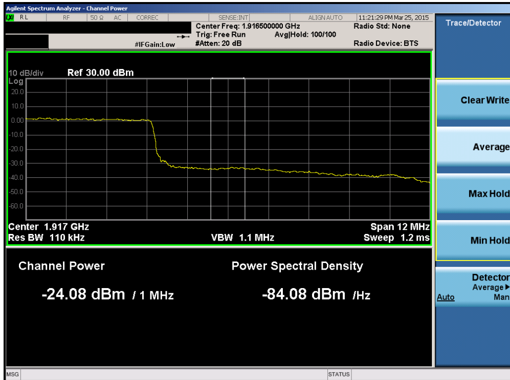
Plot 6-167. Upper Extended Band Edge Plot (Band 25 – 15.0MHz QPSK – RB Size 75)
