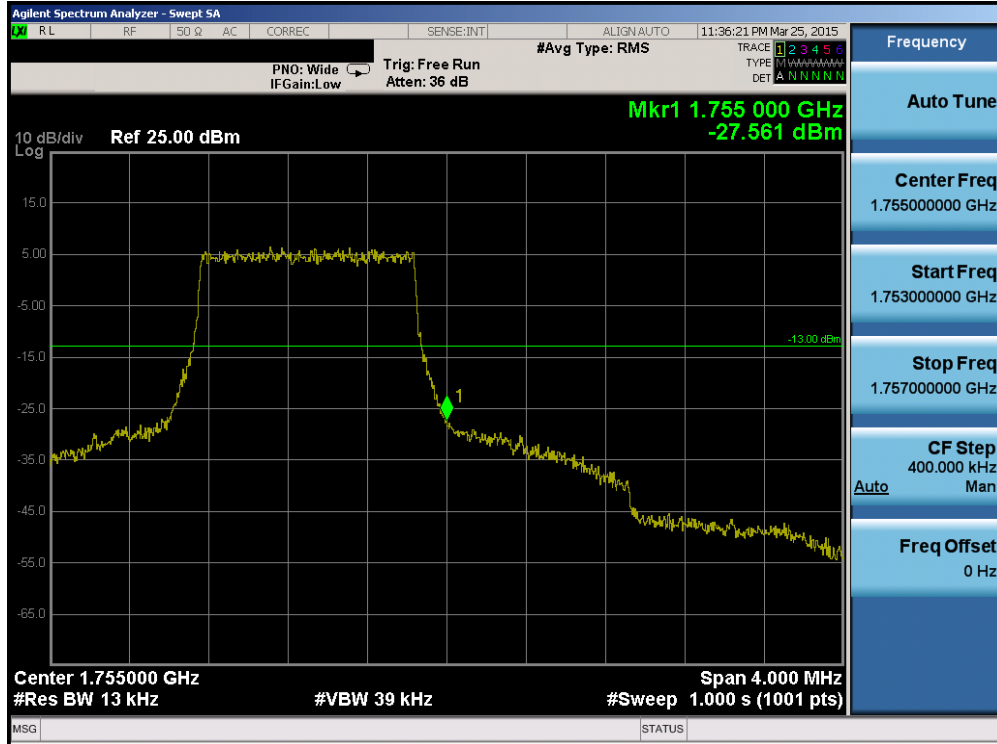
Plot 6-126. Upper Band Edge Plot (Band 4 – 1.4MHz QPSK – RB Size 6)
