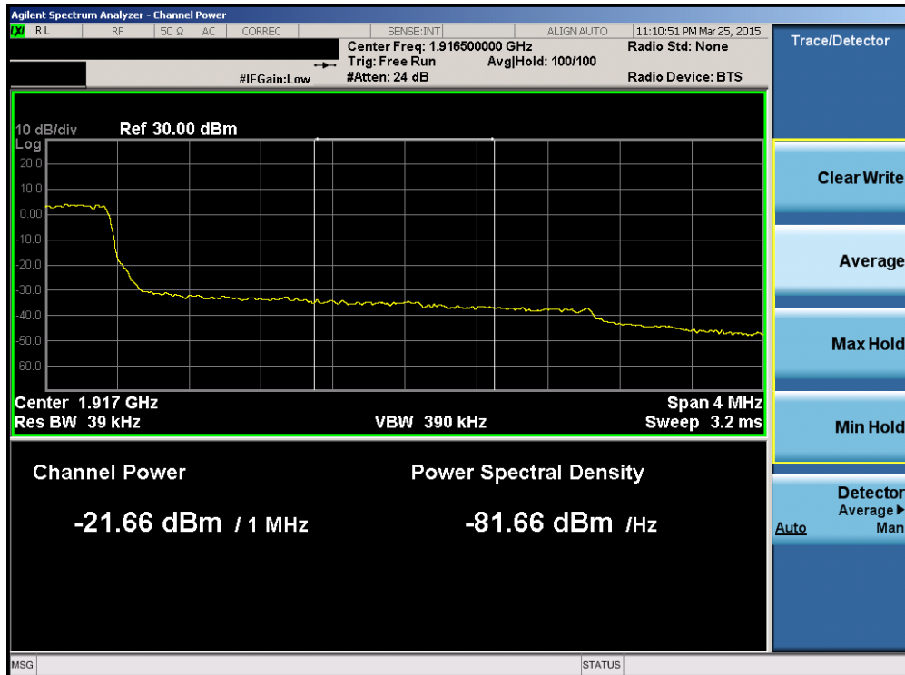
Plot 6-155. Upper Extended Band Edge Plot (Band 25 – 3.0MHz QPSK – RB Size 15)
