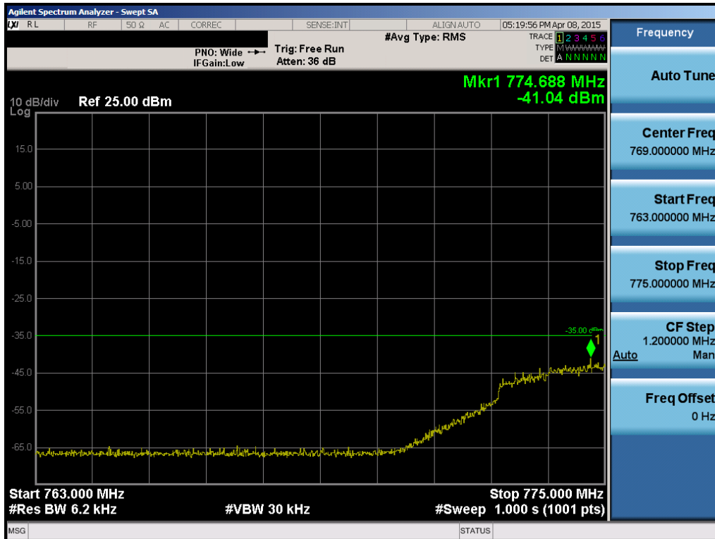
Plot 6-99. Lower Emission Mask Edge Plot (Band 13 – 5.0MHz QPSK – RB Size 25)
