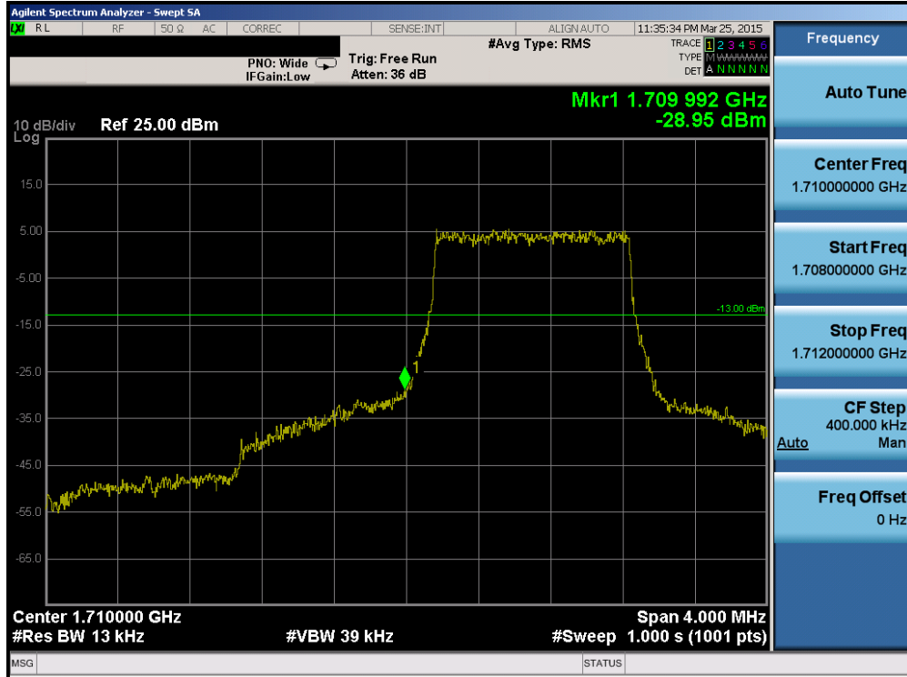
Plot 6-124. Lower Band Edge Plot (Band 4 – 1.4MHz QPSK – RB Size 6)
