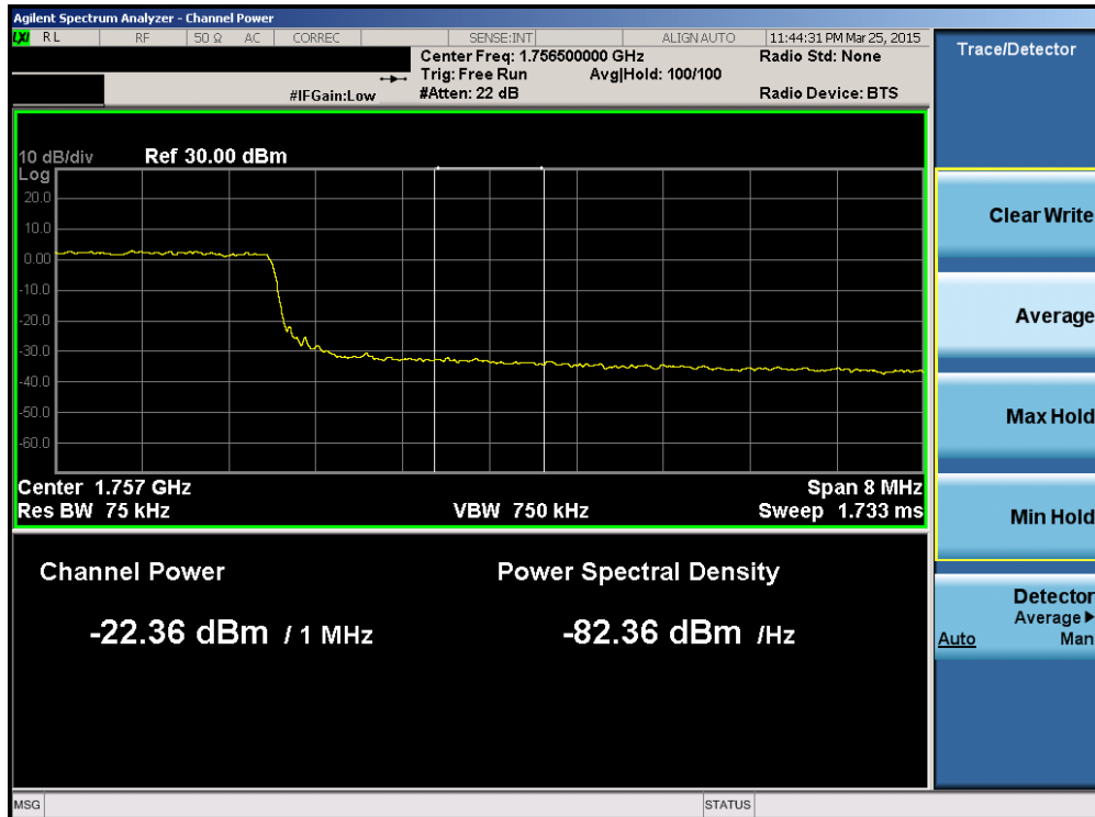
Plot 6-139. Upper Extended Band Edge Plot (Band 4 – 10.0MHz QPSK – RB Size 50)
