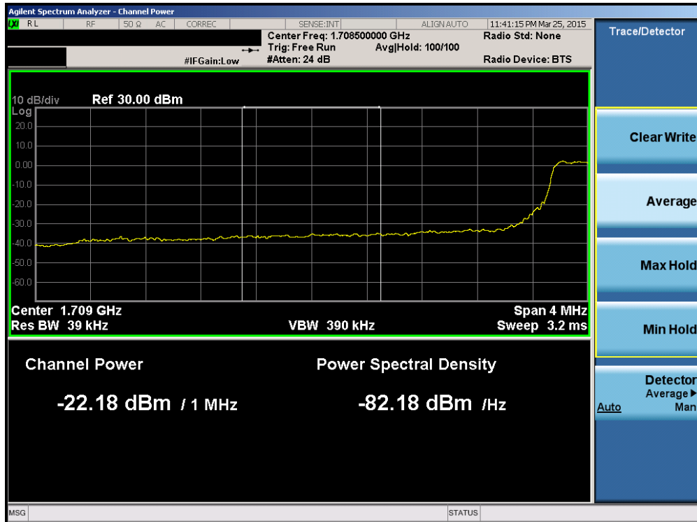
Plot 6-133. Lower Extended Band Edge Plot (Band 4 – 5.0MHz QPSK – RB Size 25)
