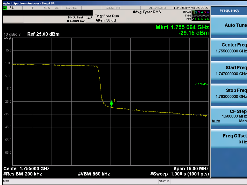
Plot 6-146. Upper Band Edge Plot (Band 4 – 20.0MHz QPSK – RB Size 100)
