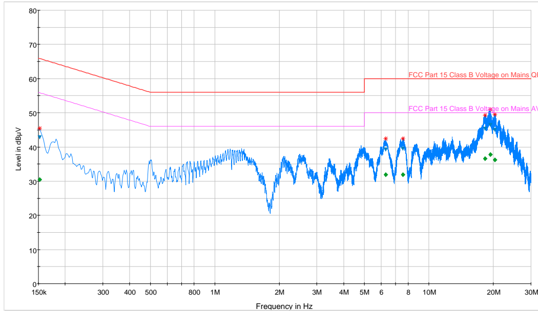
— Preview Result 1-PK+ * Critical_Freqs PK+ Final_Result QPK — FCC Part 15 Class B Voltage on Mains QP — FCC Part 15 Class B Voltage on Mains AV ◆ Final_Result AVG
