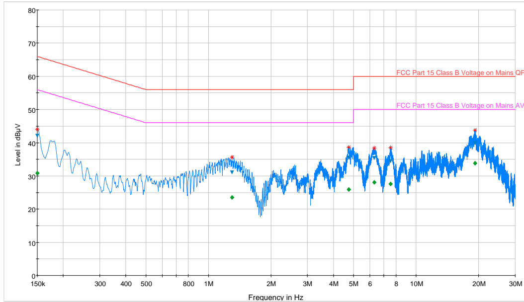
— Preview Result 1-PK+ * Critical_Freqs PK+ Final_Result QPK — FCC Part 15 Class B Voltage on Mains QP — FCC Part 15 Class B Voltage on Mains AV ▼ Final_Result QPK ◆ Final_Result AVG
