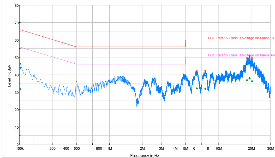
Plot 6-44. Line Conducted Plot with 802.11b (N)
