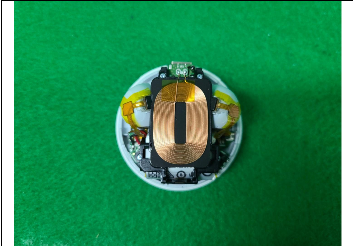
<Bluetooth Earbud (Cradle) Antenna View>
