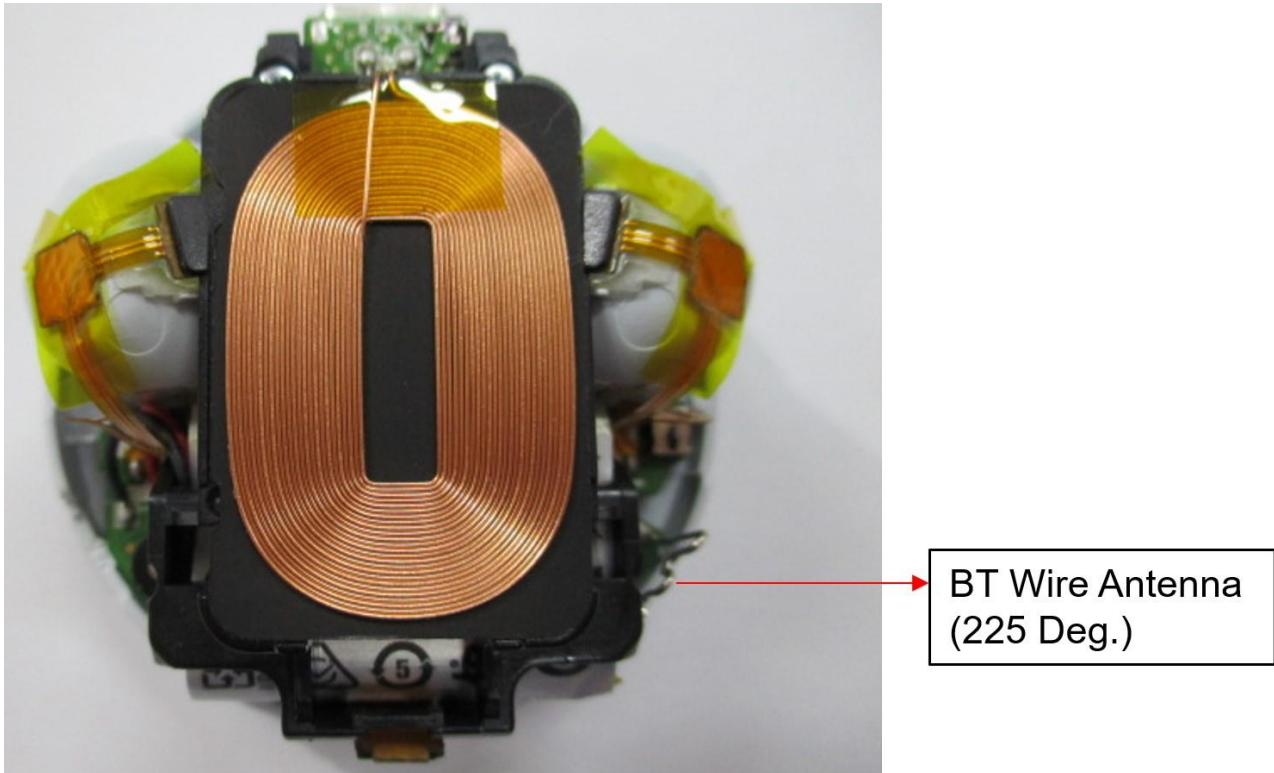
Figure E-1 Antenna Location (Rear Side View)
