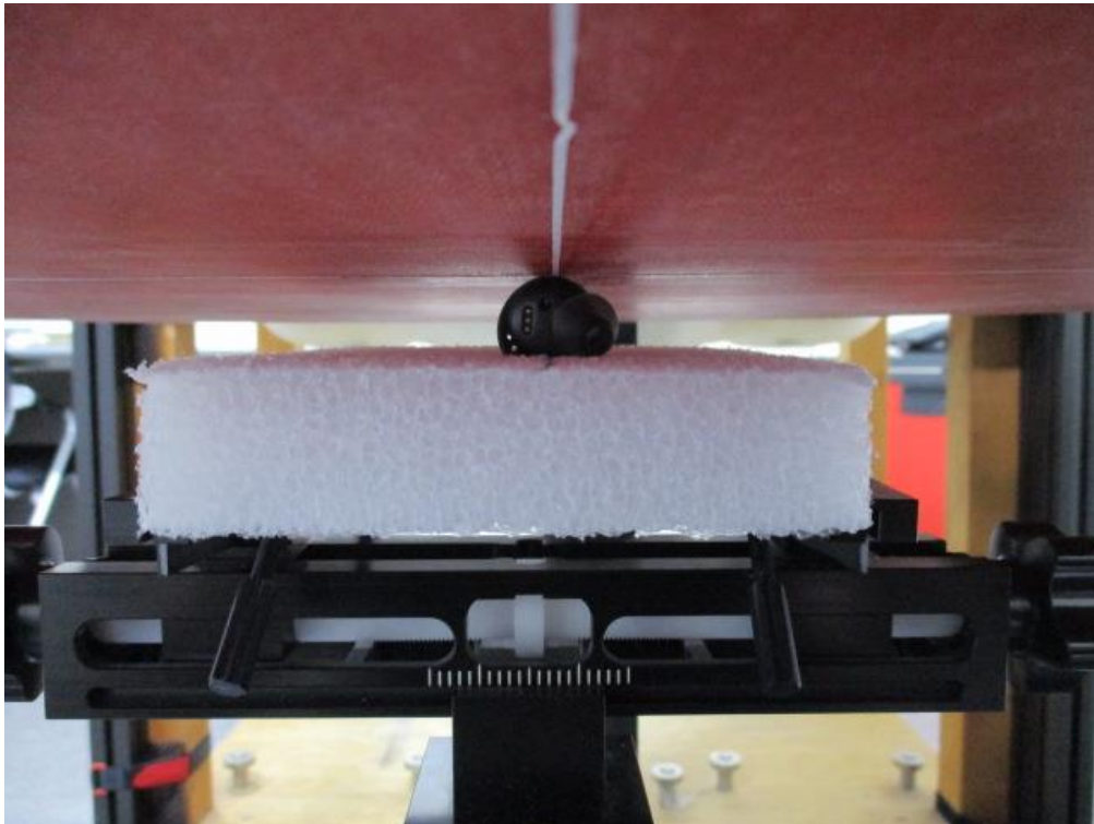
Bottom Side from Flat Phantom (Separation Distance: 0 cm) – Right Ear
