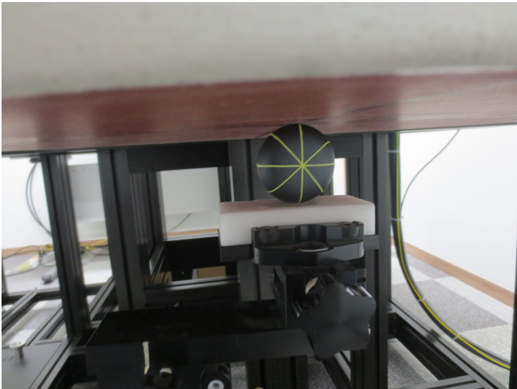
315 Deg. from Flat Phantom (Separation Distance: 0 cm)
