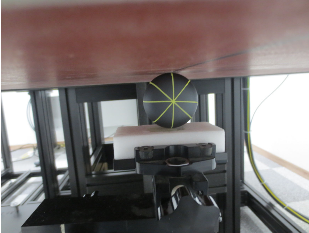
225 Deg. from Flat Phantom (Separation Distance: 0 cm)
