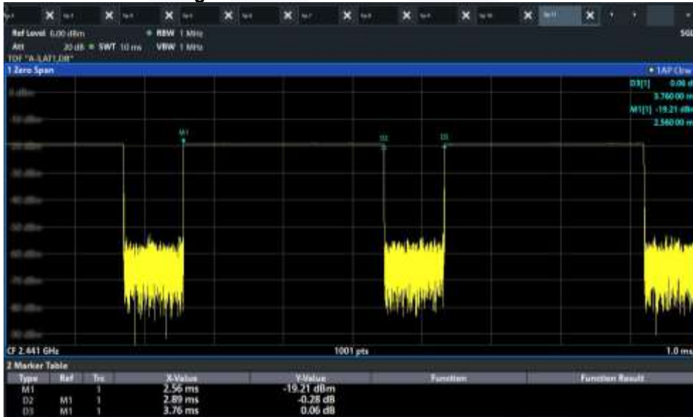
Figure 7-1 Bluetooth Transmission Plot
