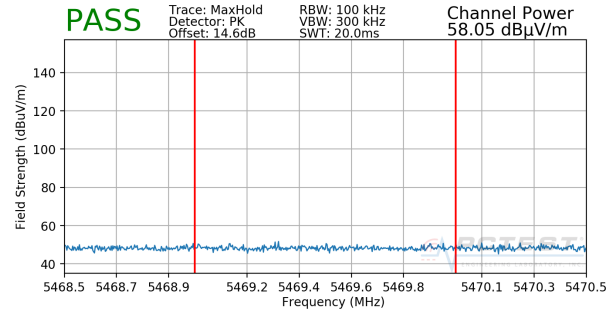
Plot 7-229. Radiated Lower Band Edge Plot MIMO (Peak – UNII Band 2C)
