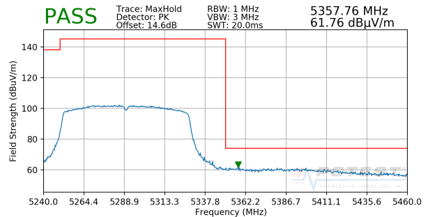
Plot 7-234. Radiated Upper Band Edge Plot MIMO (Peak – UNII Band 2A)
