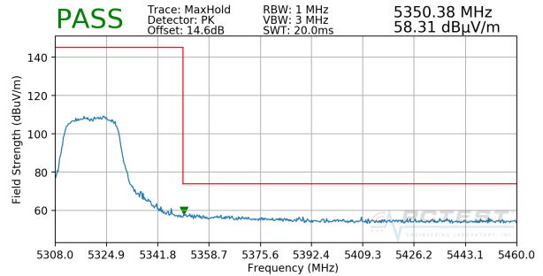
Plot 7-178. Radiated Upper Band Edge Plot SISO ANT1 (Peak – UNII Band 2A)
