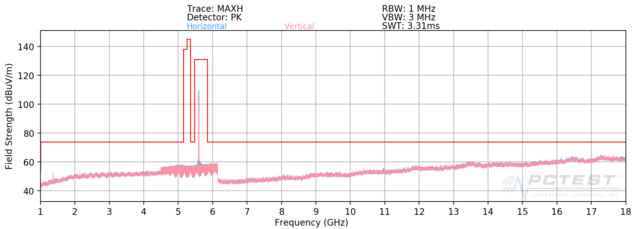
Plot 7-165. Radiated Spurious Plot above 1GHz SISO ANT2 (802.11a – U2C Ch. 120)
