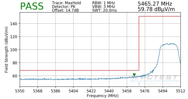
Plot 7-180. Radiated Lower Band Edge Plot SISO ANT1 (Peak – UNII Band 2C)
