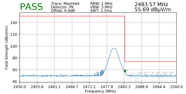
Plot 7-47. Radiated Restricted Higher Band Edge Measurement (Peak)
