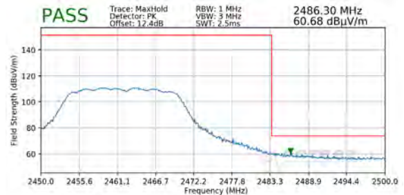
Plot 7-122. Radiated Restricted Upper Band Edge Measurement MIMO (Peak)
