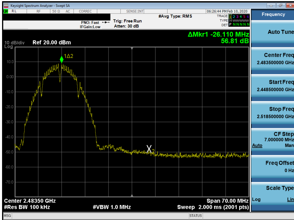
Plot 7-53. Band Edge Plot SISO ANT2 (802.11b – Ch. 11)
