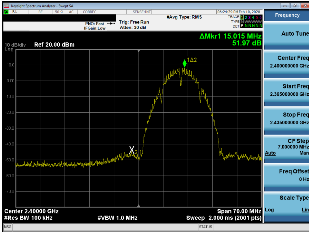
Plot 7-52. Band Edge Plot SISO ANT2 (802.11b – Ch. 1)
