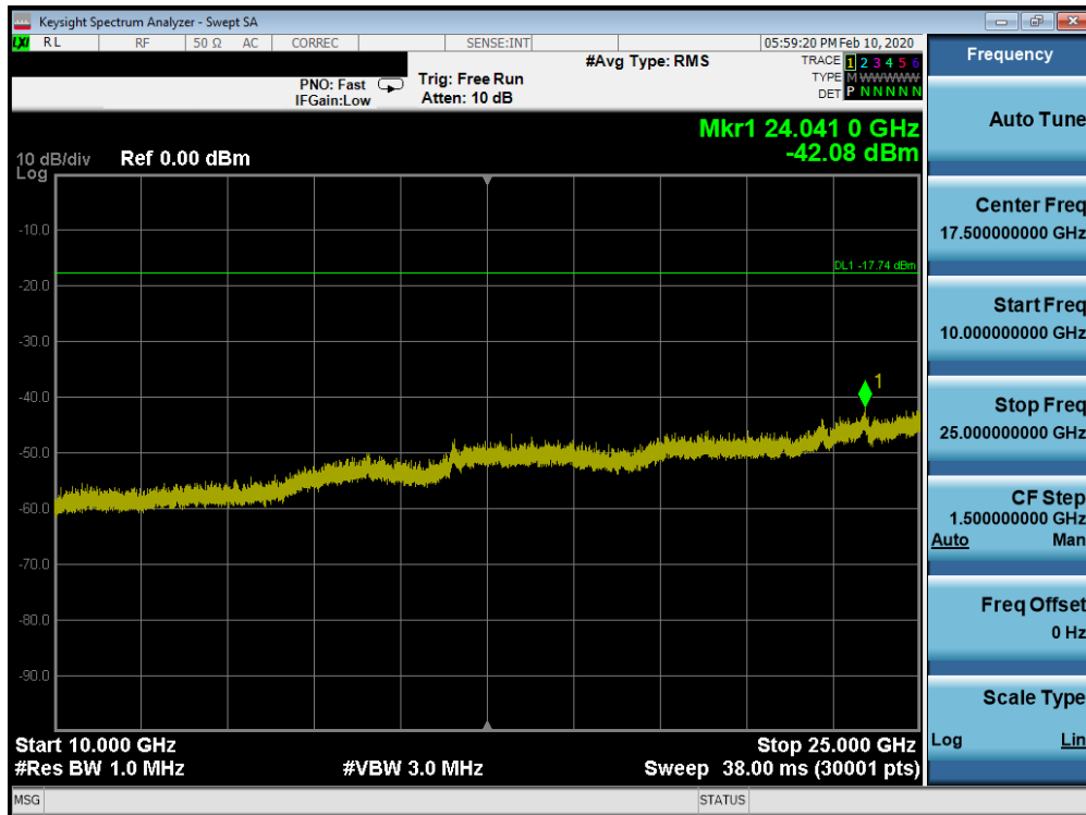
Plot 7-68. Conducted Spurious Plot SISO ANT1 (802.11b – Ch. 1)
