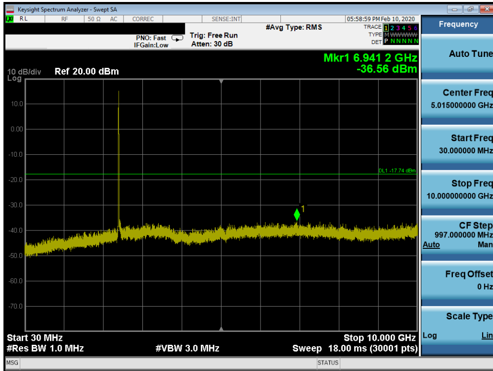
Plot 7-67. Conducted Spurious Plot SISO ANT1 (802.11b – Ch. 1)
