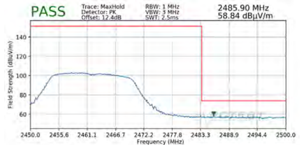
Plot 7-110. Radiated Restricted Upper Band Edge Measurement SISO ANT2 (Peak)
