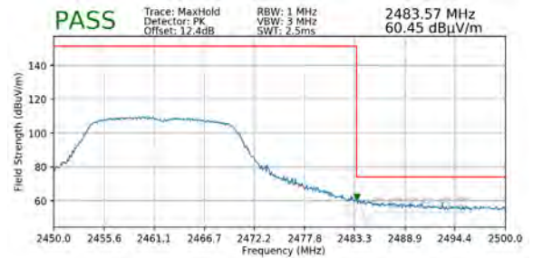
Plot 7-98. Radiated Restricted Upper Band Edge Measurement SISO ANT1 (Peak)
