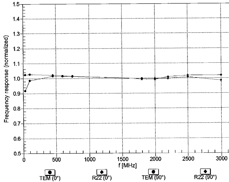
Uncertainty of Frequency Response of E-field: ± 6.3% (k=2)
