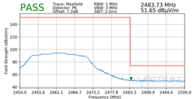
Plot 7-16. Radiated Restricted Upper Band Edge Measurement SISO ANT2 (Peak)
