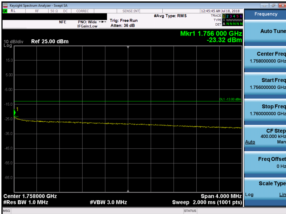
Plot 7-210. Upper Extended Band Edge Plot (Band 4 - 10.0MHz QPSK - Full RB Configuration)
