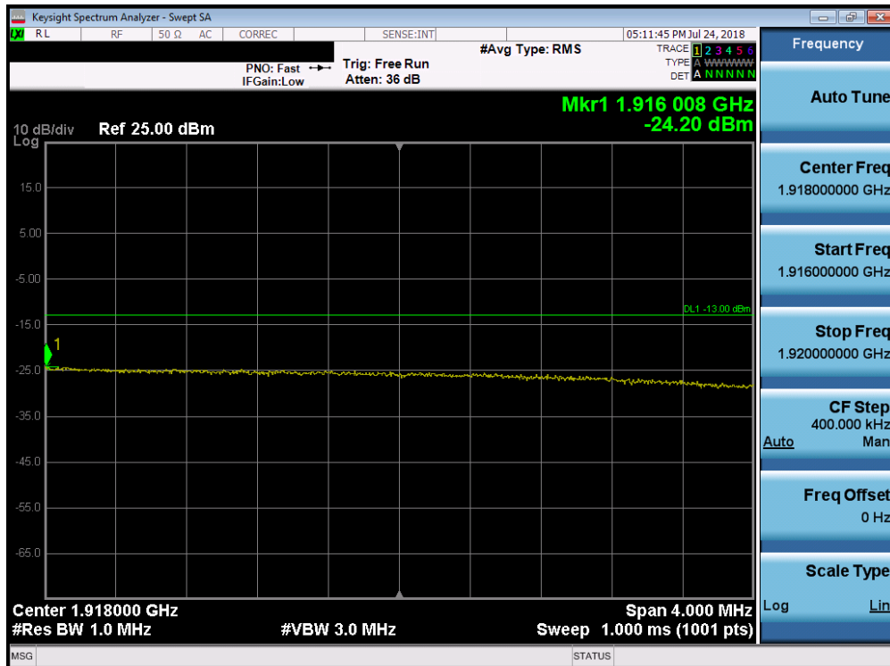
Plot 7-254. Upper Extended Band Edge Plot (Band 25 - 15.0MHz QPSK - Full RB Configuration)
