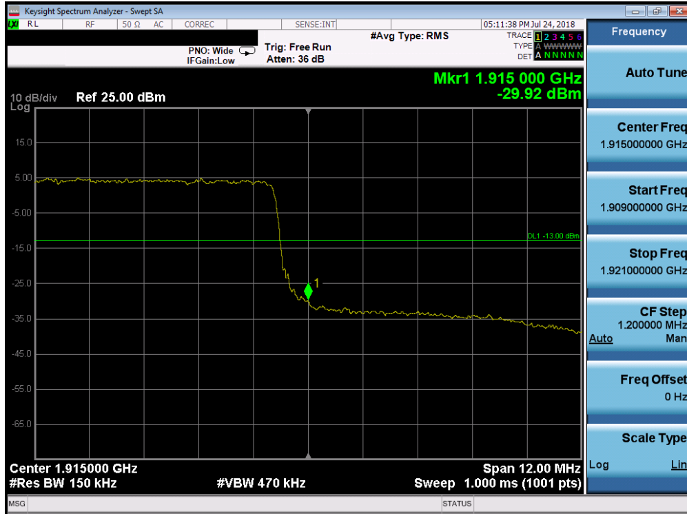
Plot 7-253. Upper Band Edge Plot (Band 25 - 15.0MHz QPSK - Full RB Configuration)
