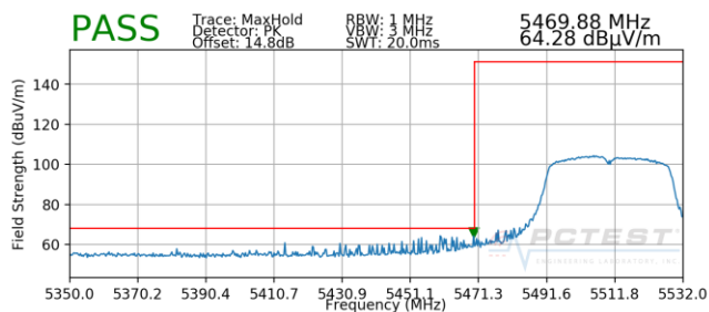
Plot 7-202. Radiated Lower Band Edge Plot SISO ANT2 (Peak – UNII Band 2C)
