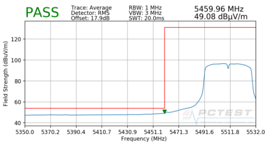
Plot 7-201. Radiated Lower Band Edge Plot SISO ANT2 (Average – UNII Band 2C)
