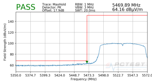
Plot 7-209. Radiated Lower Band Edge Plot SISO ANT2 (Peak – UNII Band 2C)
