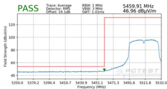
Plot 7-222. Radiated Lower Band Edge Plot MIMO (Average – UNII Band 2C)
