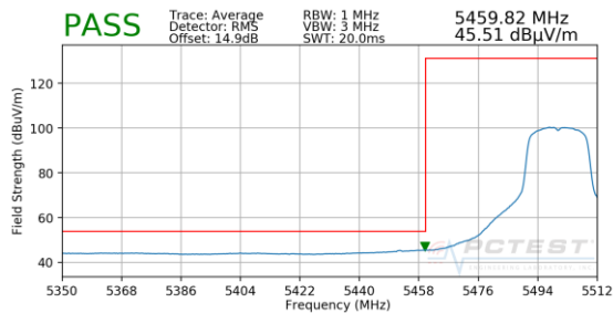
Plot 7-194. Radiated Lower Band Edge Plot SISO ANT2 (Average – UNII Band 2C)
