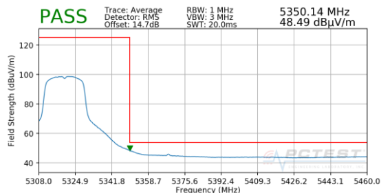
Plot 7-192. Radiated Upper Band Edge Plot SISO ANT2 (Average – UNII Band 2A)
