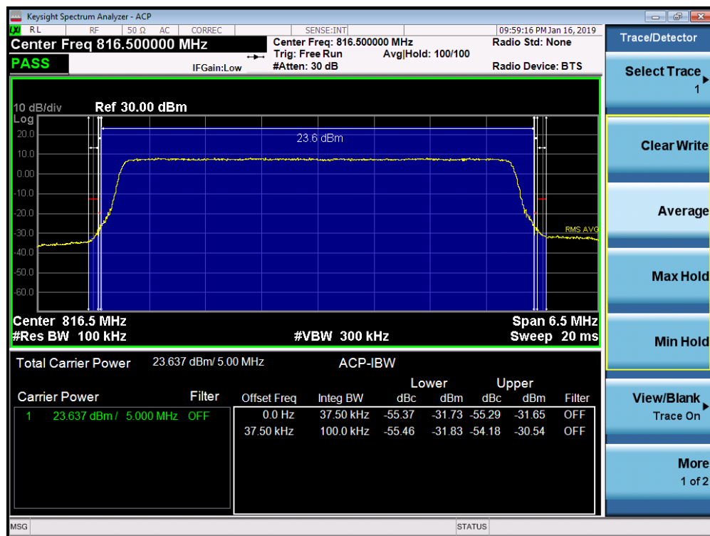
Plot 7-34. Channel Edge Plot (LTE Band 26, 5MHz QPSK – RB Size 25– Low Channel)
