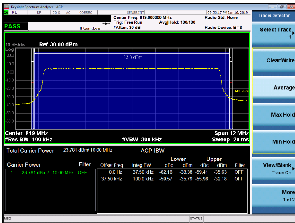
Plot 7-36. Channel Edge Plot (LTE Band 26, 10MHz QPSK – RB Size 50)
