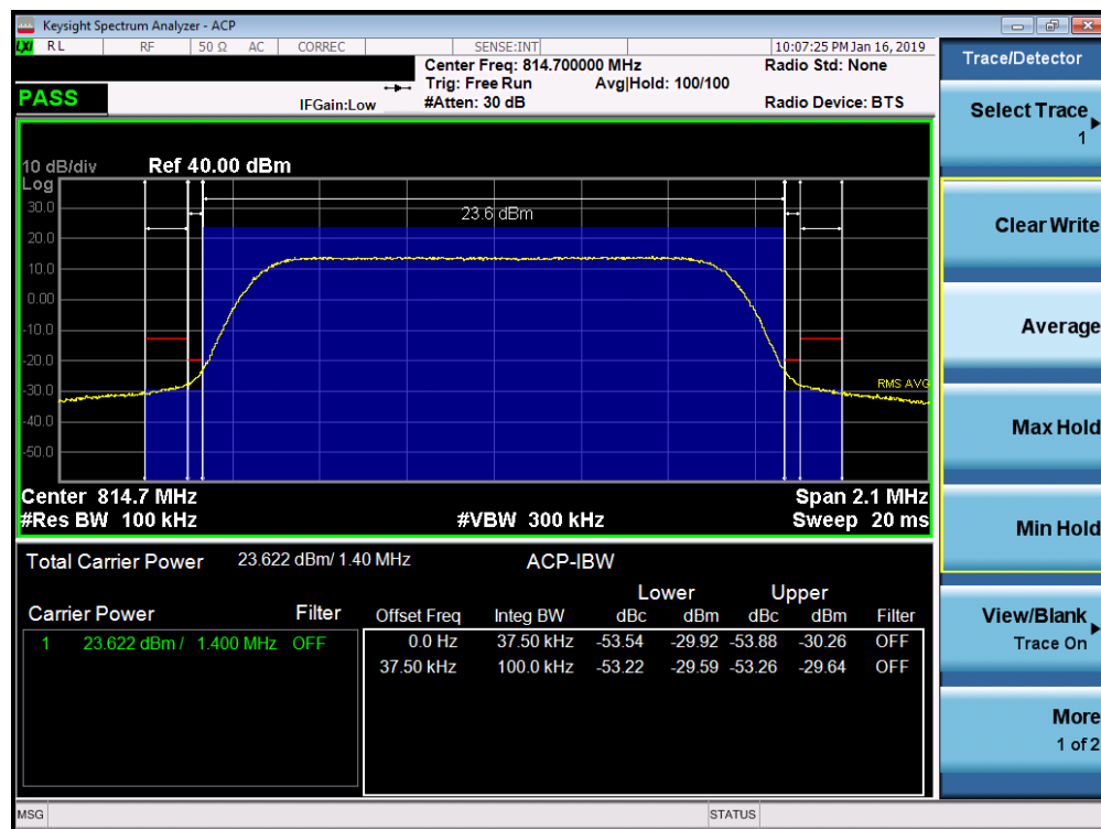
Plot 7-30. Channel Edge Plot (LTE Band 26, 1.4MHz QPSK - RB Size 6- Low Channel)
