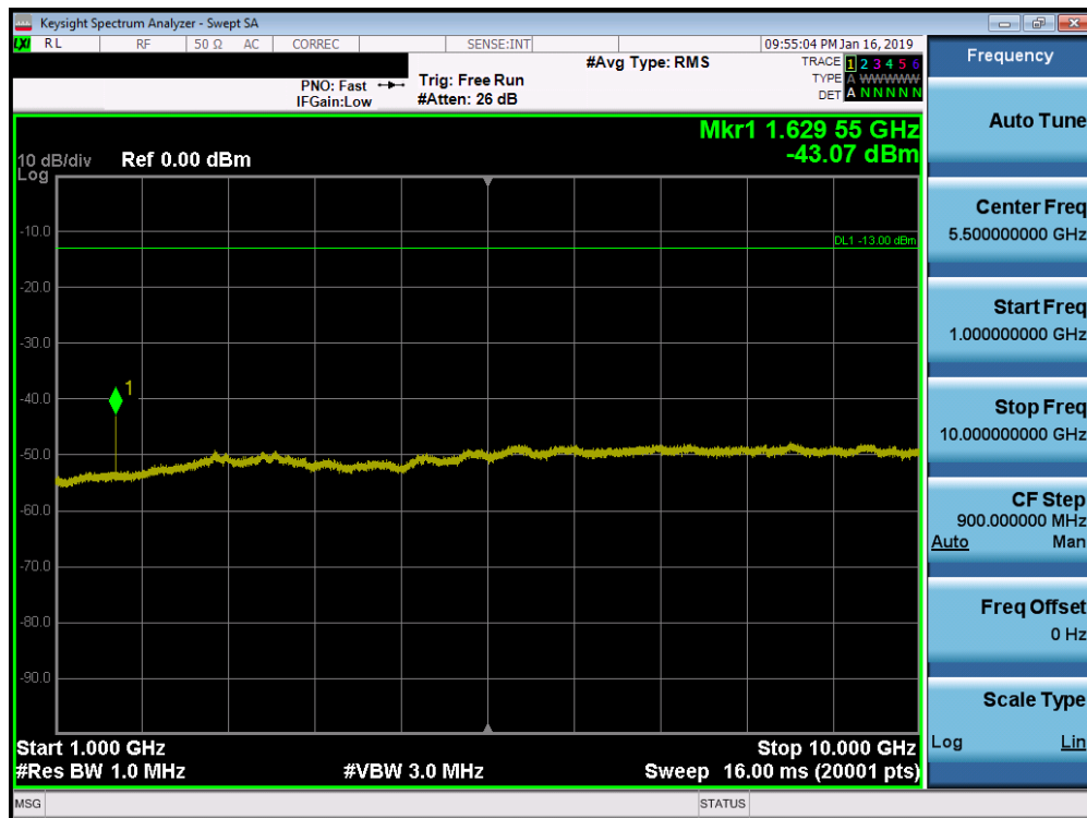
Plot 7-26. Conducted Spurious Plot (LTE Band 26, 10MHz QPSK – RB Size 1, RB Offset 0 – Mid Channel)
