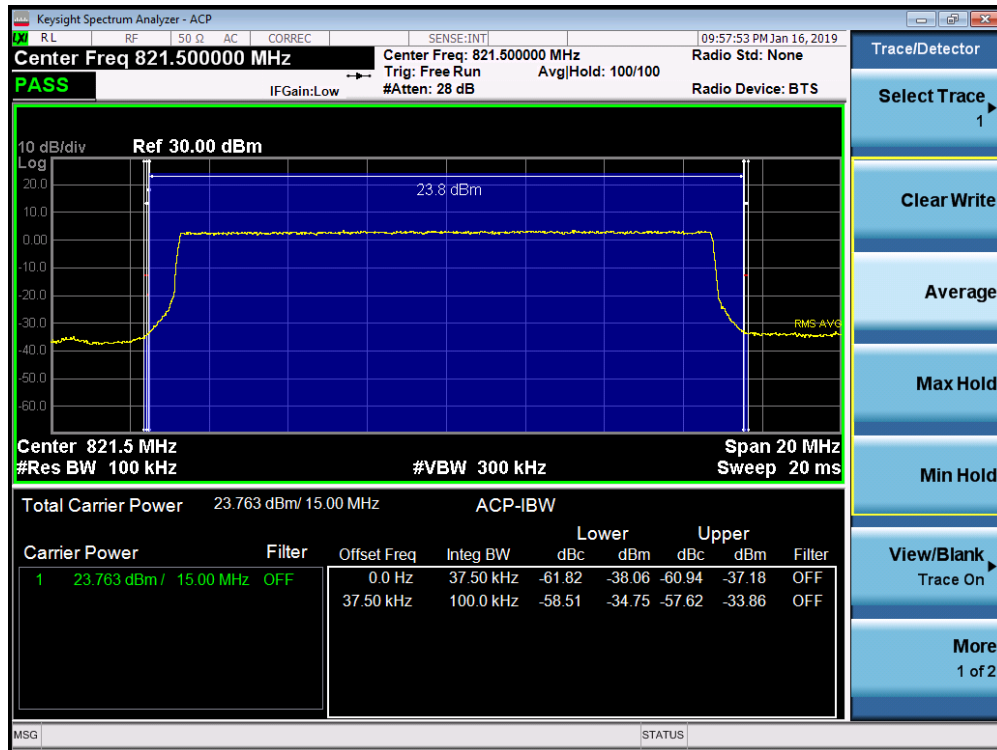
Plot 7-37. Channel Edge Plot (LTE Band 26, 15MHz QPSK – RB Size 75)
