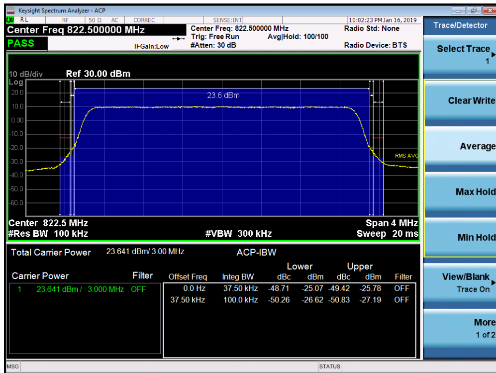
Plot 7-33. Channel Edge Plot (LTE Band 26, 3MHz QPSK – RB Size 15 – High Channel)
