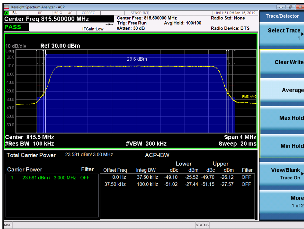
Plot 7-32. Channel Edge Plot (LTE Band 26, 3MHz QPSK – RB Size 15– Low Channel)
