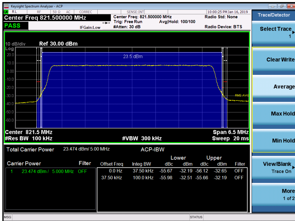
Plot 7-35. Channel Edge Plot (LTE Band 26, 5MHz QPSK – RB Size 25 – High Channel)
