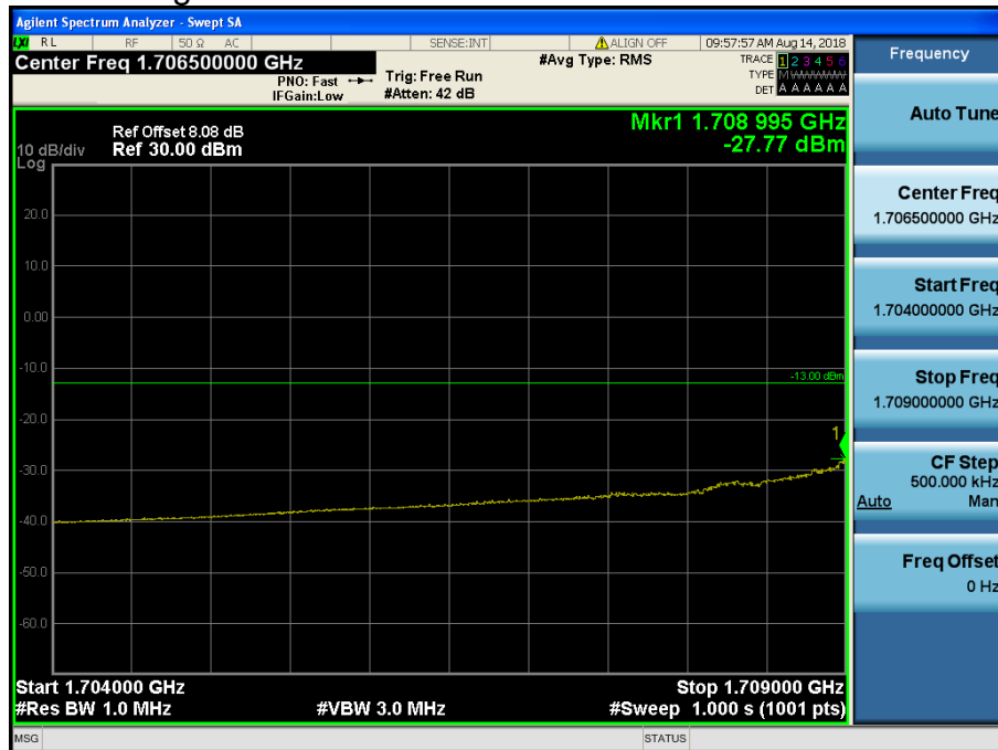
LTE Band 4,66 / 3MHz / QPSK - RB Size/Offset (8/4)
