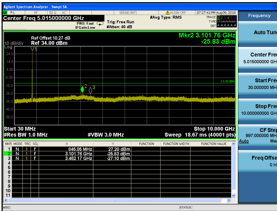
LTE Band 5 / 10MHz / QPSK - RB Size/Offset (25/25) – High Channel
