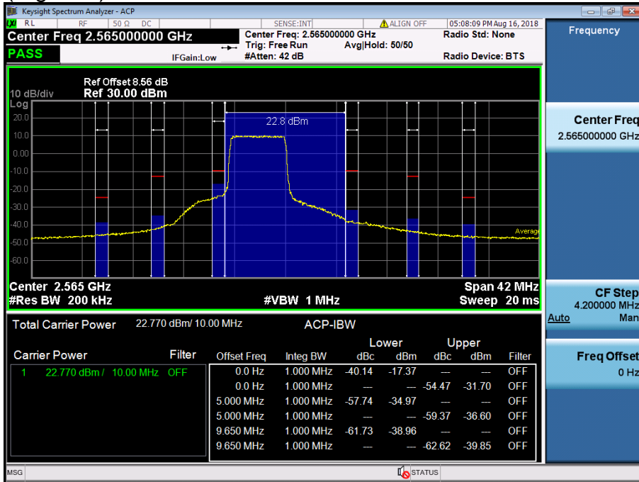
LTE Band 7 / 10MHz / 16QAM - RB Size/Offset (25/0)
