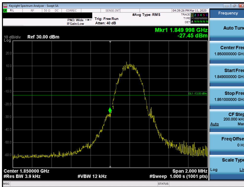
Plot 7-55. Band Edge Plot (PCS GPRS Mode - Low Channel)
