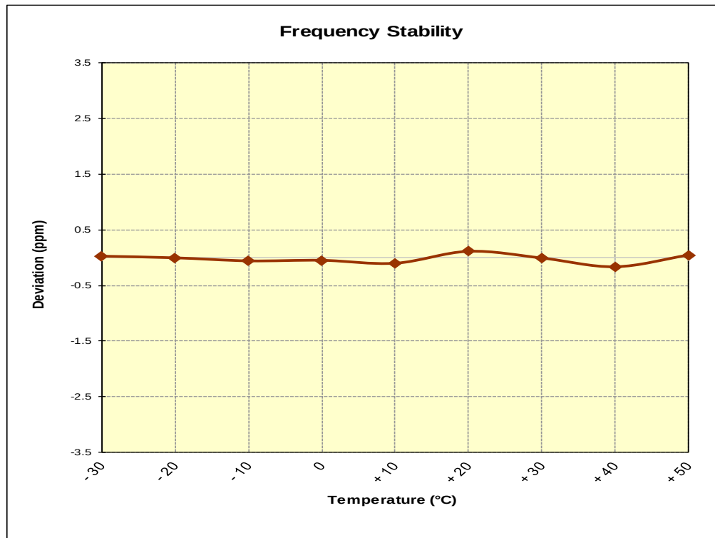
Figure 7-12. Frequency Stability Graph (PCS GPRS Mode – Ch. 661)
