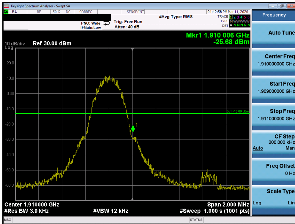
Plot 7-57. Band Edge Plot (PCS GPRS Mode - High Channel)
