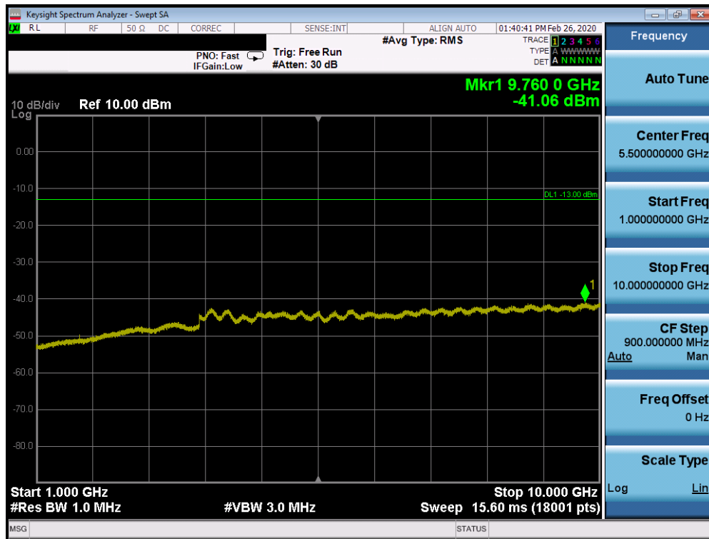
Plot 7-34. Conducted Spurious Plot (Cellular WCDMA Mode - High Channel)
