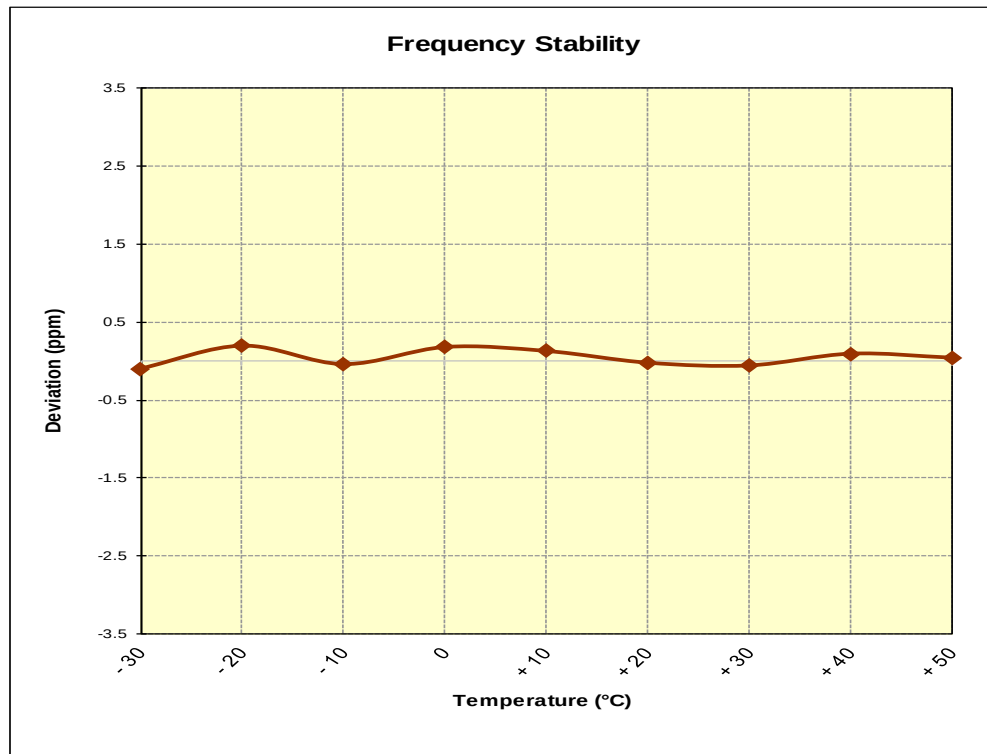
Figure 7-13. Frequency Stability Graph (PCS WCDMA Mode – Ch. 9400)
