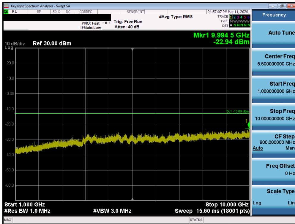
Plot 7-10. Conducted Spurious Plot (Cellular GPRS Mode - Low Channel)
