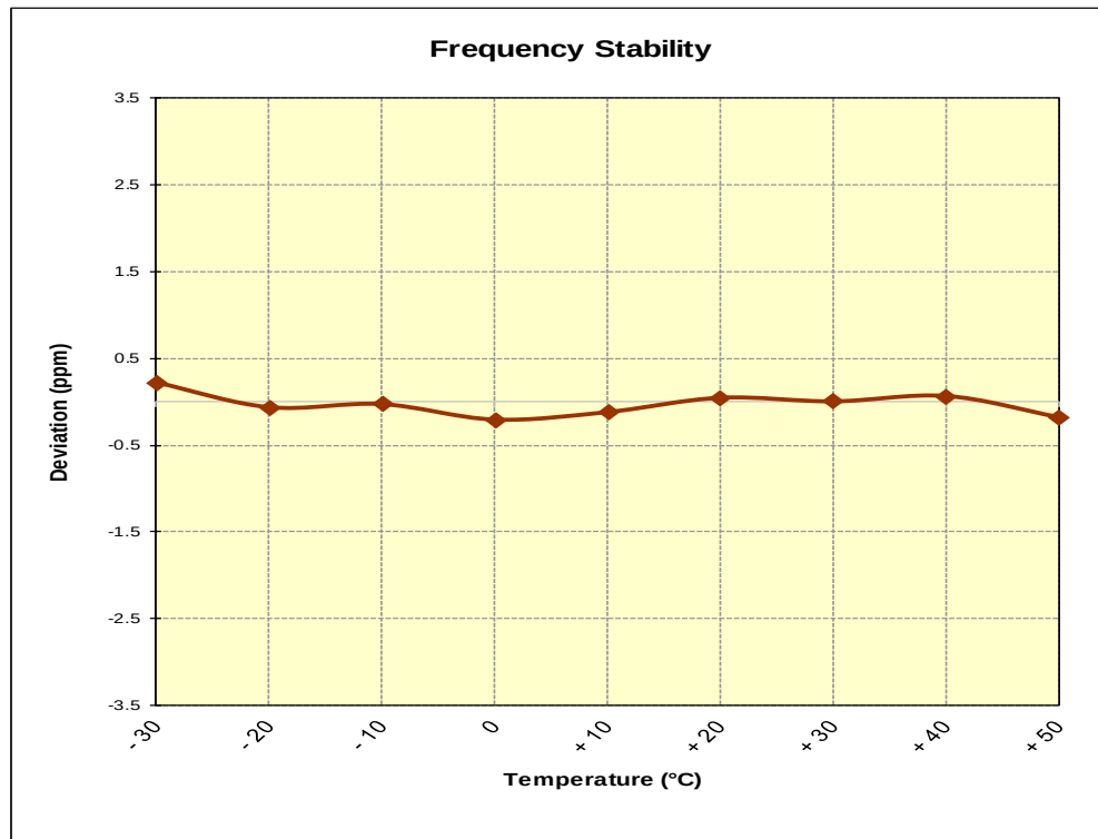
Figure 7-11. Frequency Stability Graph (AWS WCDMA Mode – Ch. 1413)
