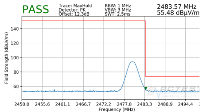
Plot 7-19. Radiated Restricted Upper Band Edge Measurement (Peak)
