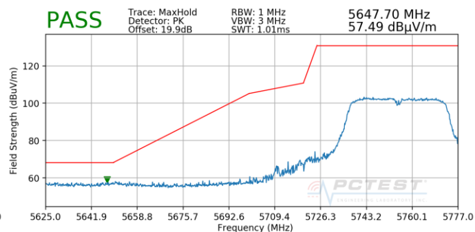
Plot 7-113. Radiated Lower Band Edge Plot (Peak – UNII Band 3)
