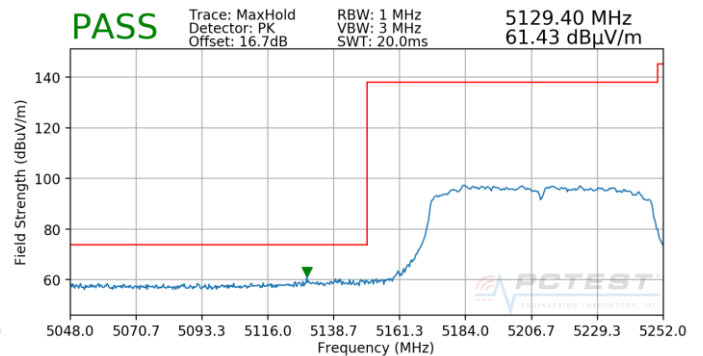
Plot 7-116. Radiated Lower Band Edge Plot (Peak – UNII Band 1)
