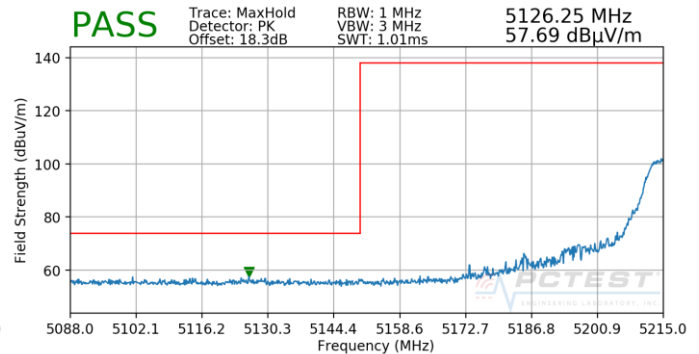
Plot 7-103. Radiated Lower Band Edge Plot (Peak – UNII Band 1-Interior)
