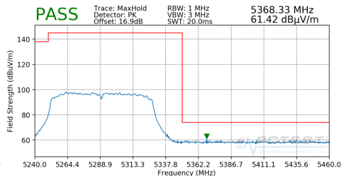
Plot 7-118. Radiated Upper Band Edge Plot (Peak – UNII Band 2A)
