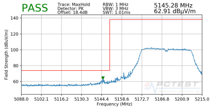
Plot 7-101. Radiated Lower Band Edge Plot (Peak – UNII Band 1)
