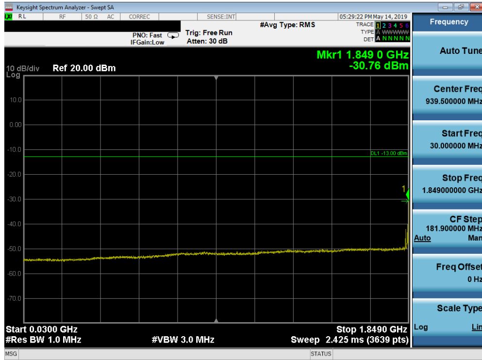
Plot 7-139. Conducted Spurious Plot (Band 25/2 - 20.0MHz QPSK - RB Size 1, RB Offset 0 - Low Channel)
