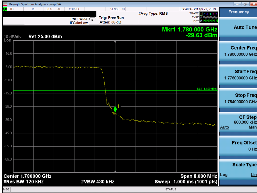
Plot 7-213. Upper Band Edge Plot (Band 66 - 10.0MHz QPSK - Full RB Configuration)
