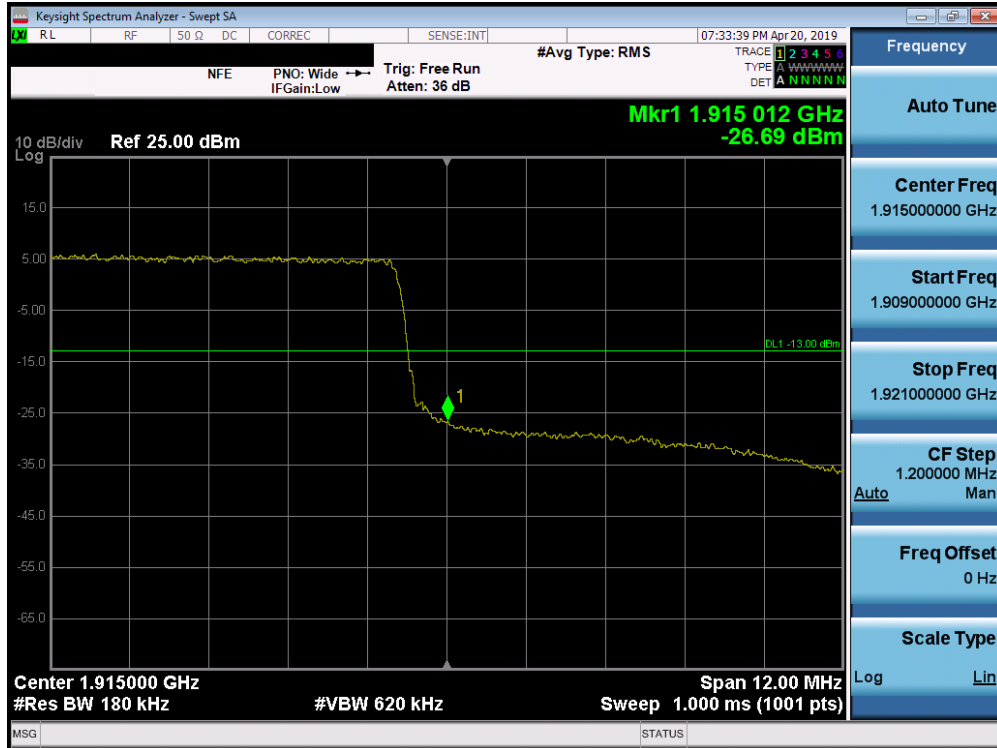
Plot 7-255. Upper Band Edge Plot (Band 25 - 15.0MHz QPSK - Full RB Configuration)
