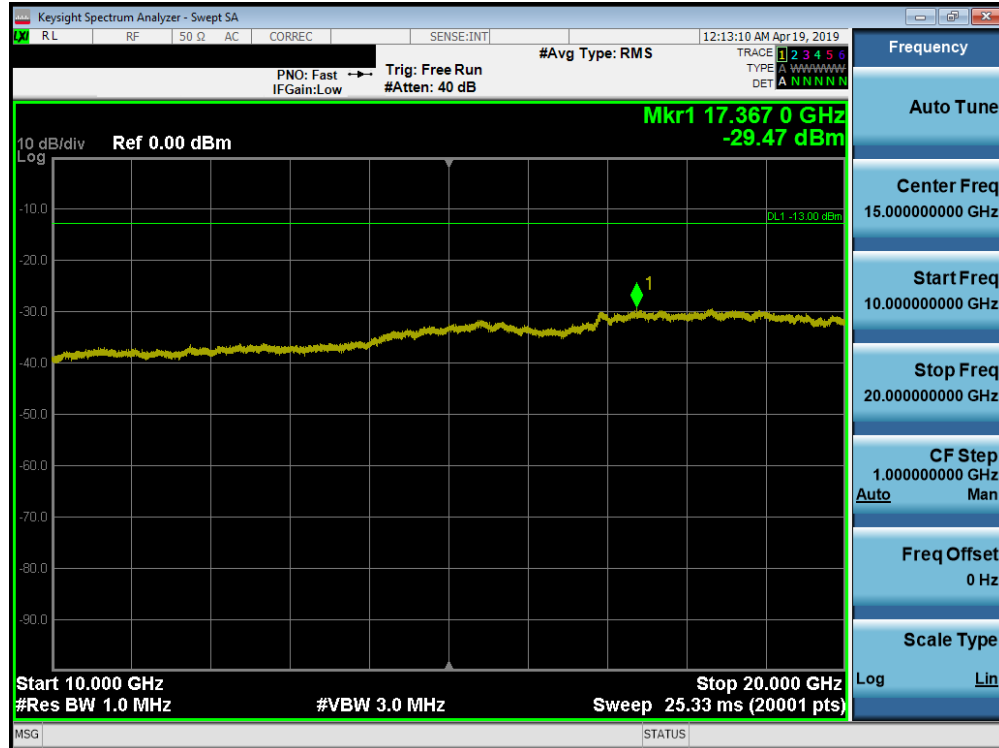
Plot 7-132. Conducted Spurious Plot (Band 66/4 - 20MHz QPSK - RB Size 1, RB Offset 0 - High Channel)
