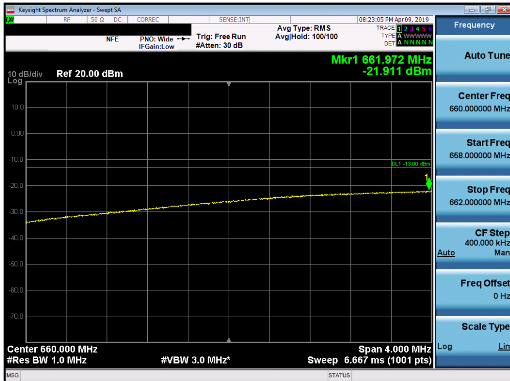
Plot 7-160. Lower Extended Band Edge Plot (Band 71 - 20.0MHz QPSK - Full RB Configuration)
