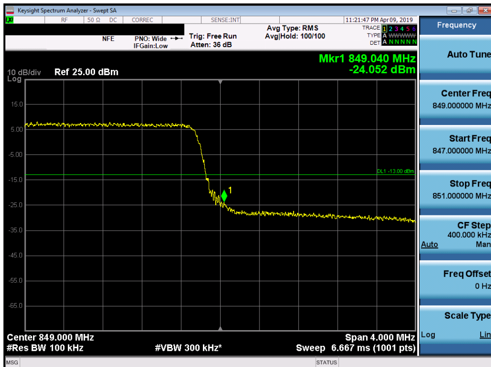
Plot 7-186. Upper Band Edge Plot (Band 26/5 - 5.0MHz QPSK - Full RB Configuration)
