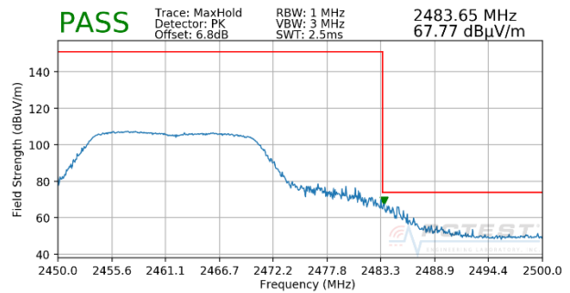
Plot 7-50. Radiated Restricted Upper Band Edge Measurement (Peak)
