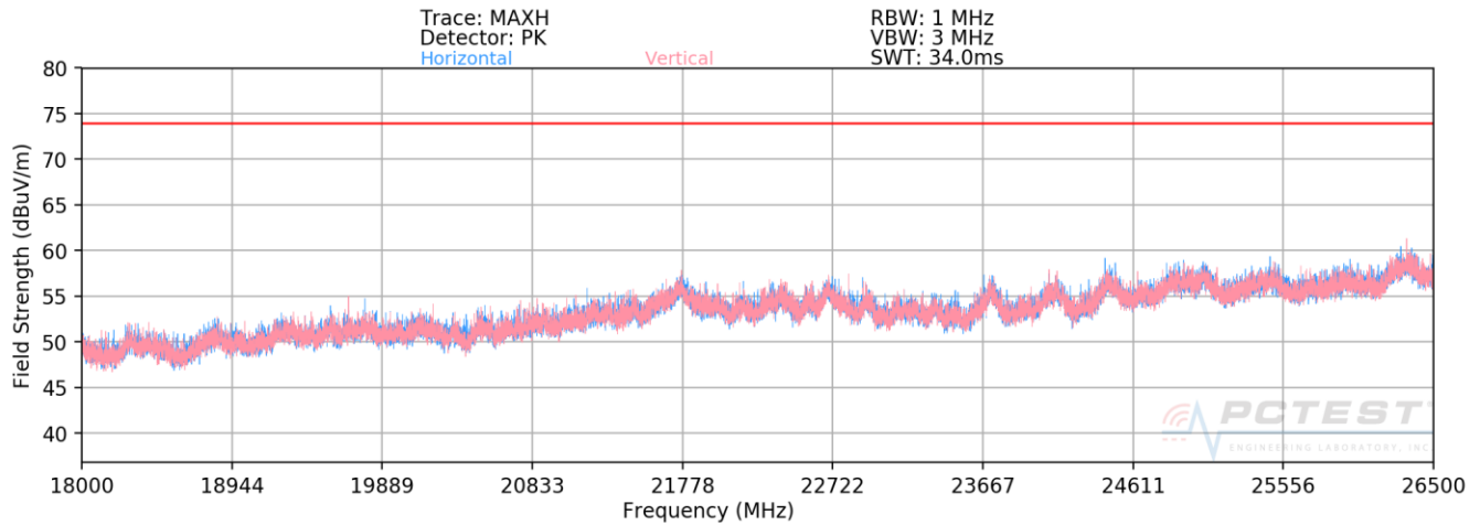
Plot 7-38. Radiated Spurious Plot above 18GHz ANT1
