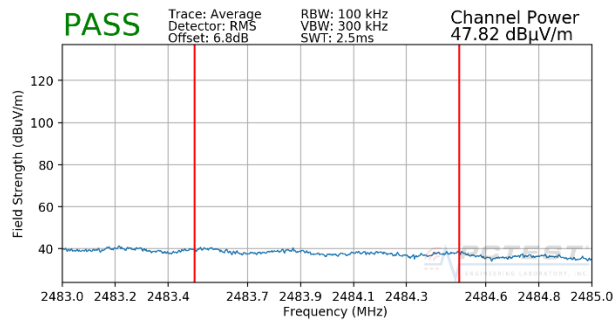
Plot 7-49. Radiated Restricted Upper Band Edge Measurement (Average)
