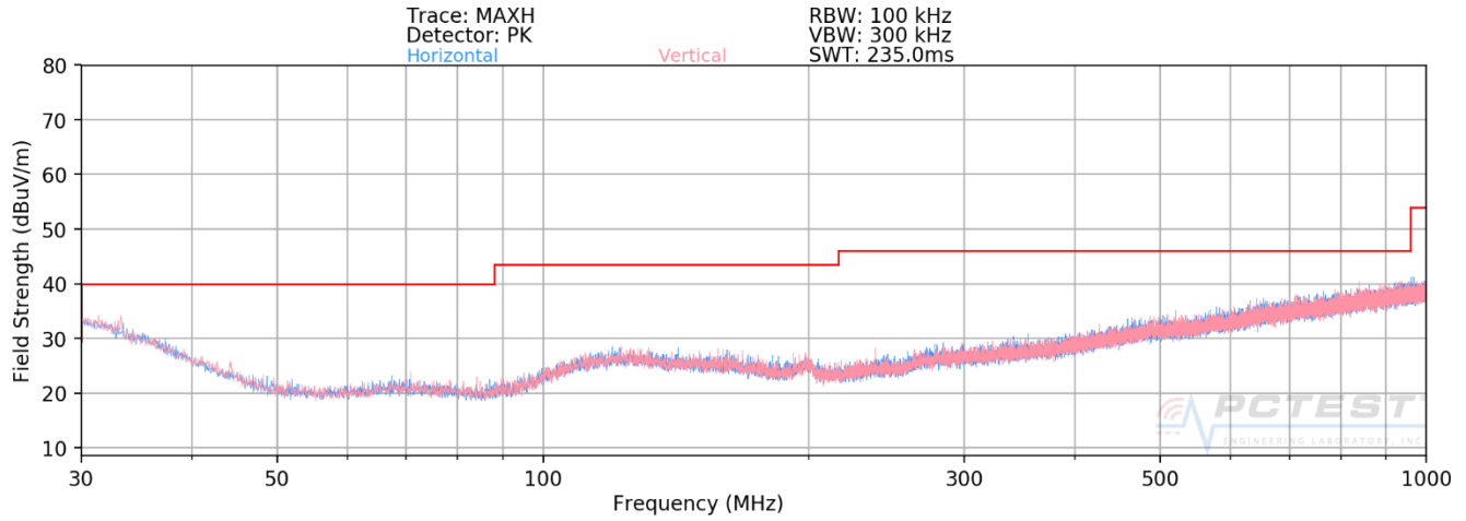
Plot 7-51. Radiated Spurious Plot below 1GHz ANT1
