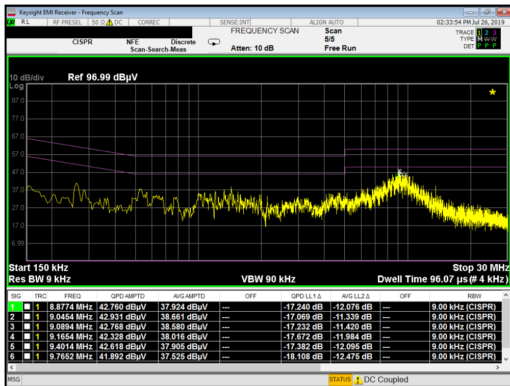
Plot 7-128. Line Conducted Plot with 802.11a UNII Band 2A (N)
