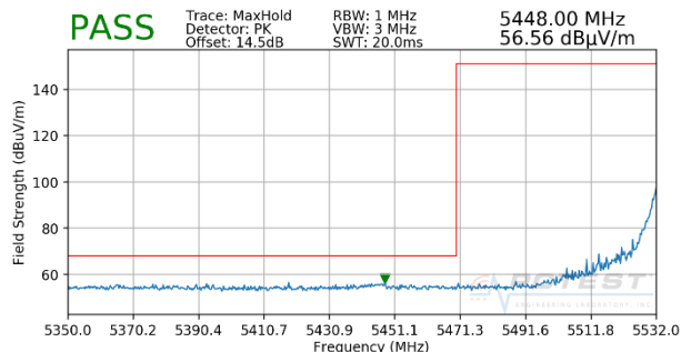
Plot 7-112. Radiated Lower Band Edge Plot (Peak – UNII Band 2C - Interior)
