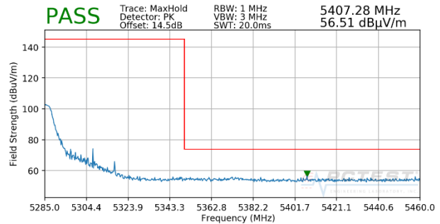
Plot 7-106. Radiated Upper Band Edge Plot (Peak – UNII Band 2A - Interior)
