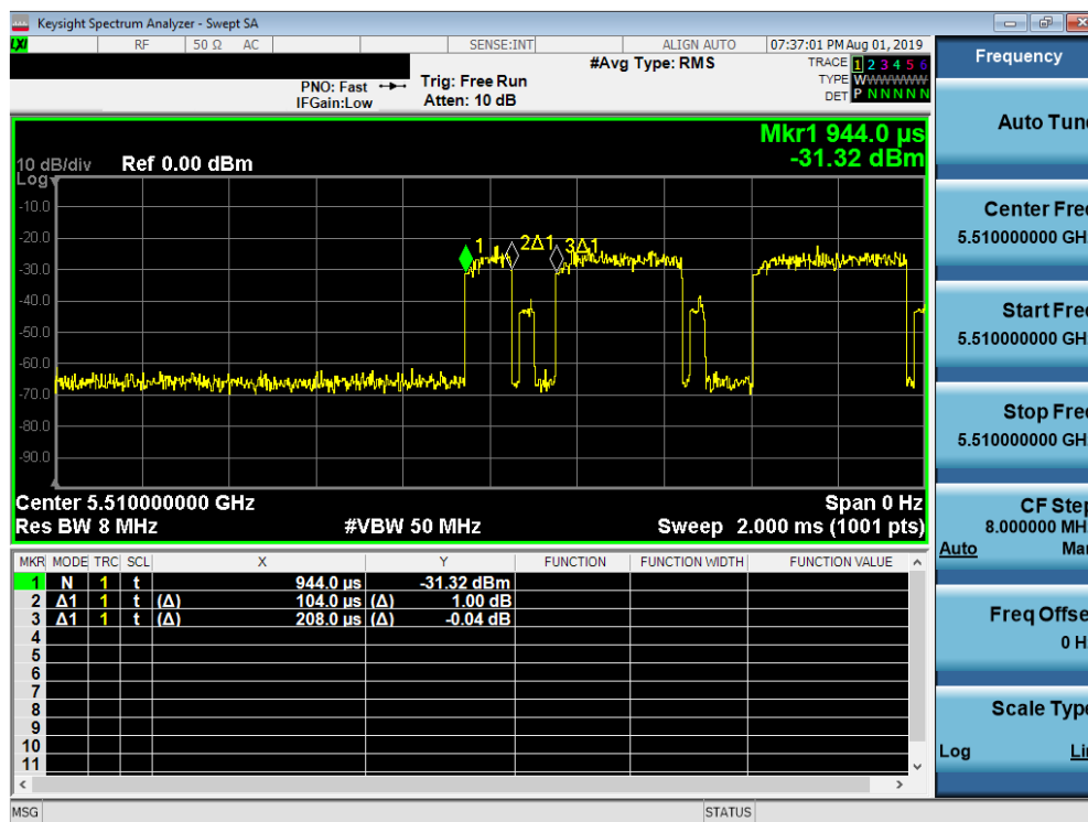
Figure 6-1. Band 2C Pulse Width and Period
