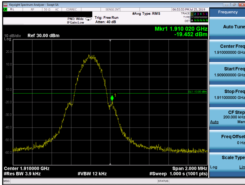
Plot 7-57. Band Edge Plot (PCS GRPS Mode - High Channel)
