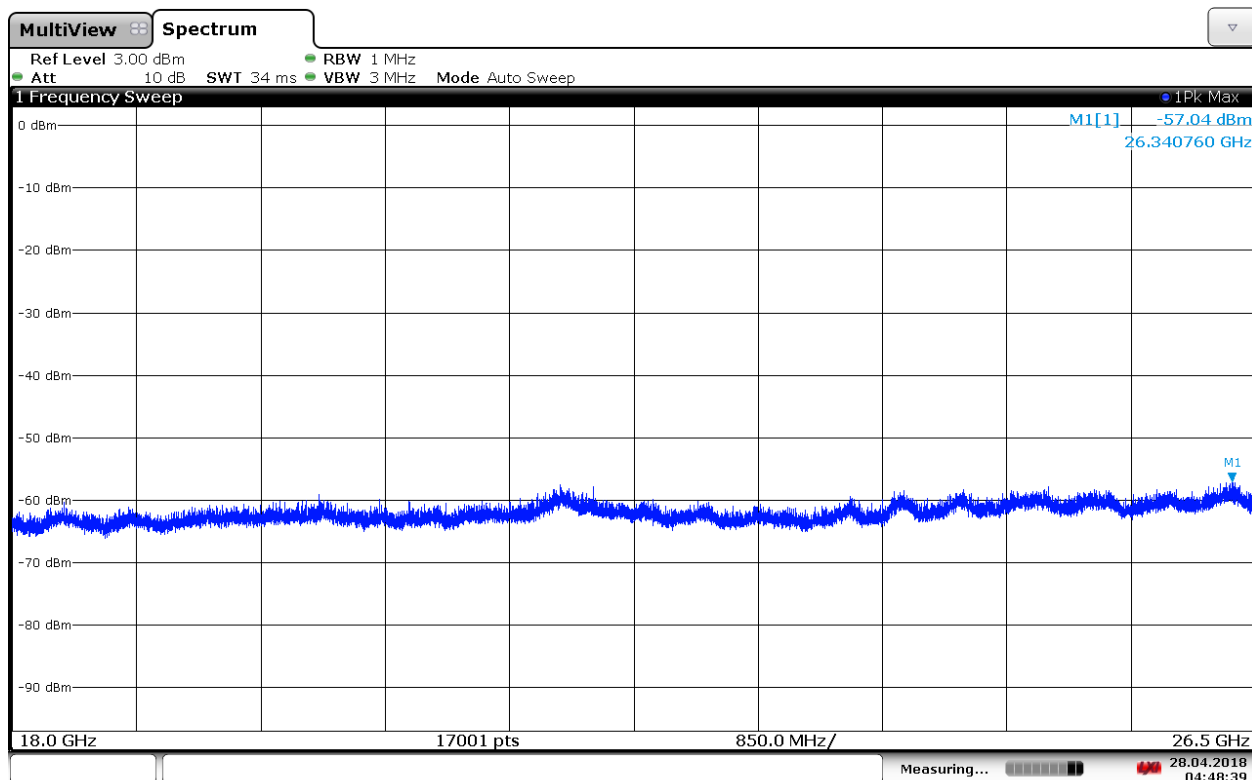
Plot 7-267. Radiated Spurious Plot 18GHz – 26.5GHz (Band 41) - Vertical
