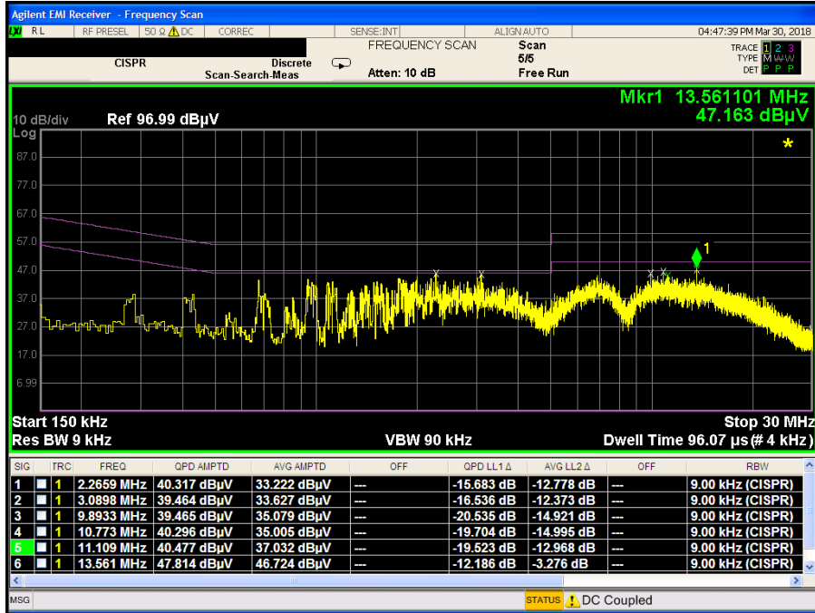
Plot 7-6. Line-Conducted Test Plot (L1)
