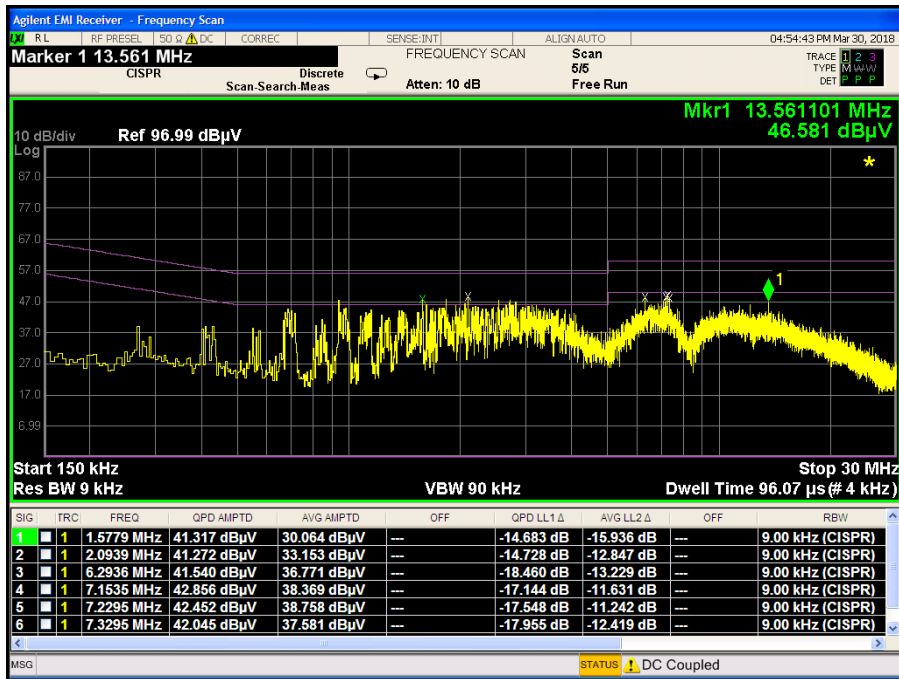
Plot 7-7. Line-Conducted Test Plot (N)
