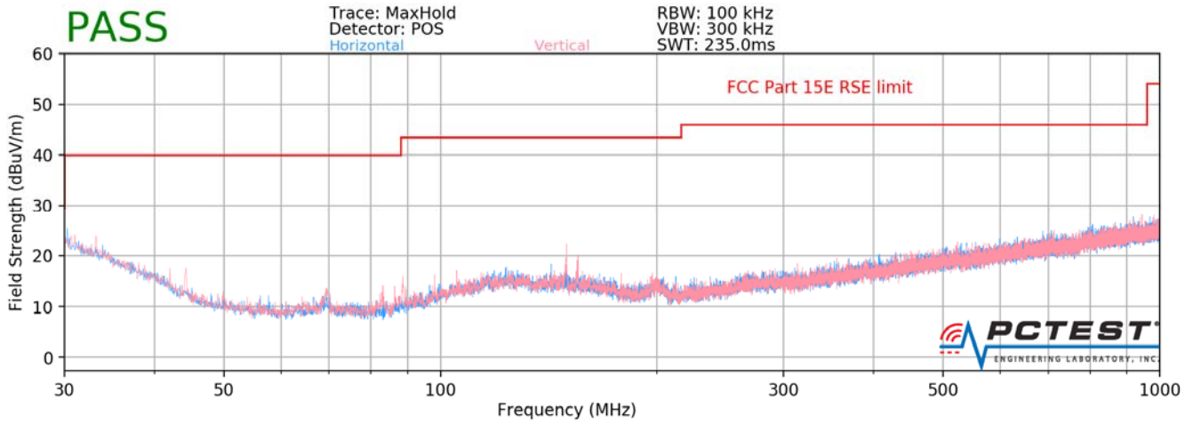
Plot 7-103. Radiated Spurious Plot below 1GHz (802.11ac – U3 Ch. 157)
