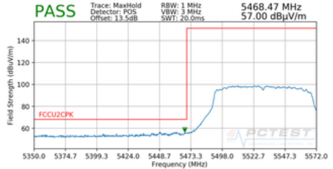
Plot 7-100. Radiated Lower Band Edge Plot (Peak – UNII Band 2C)
