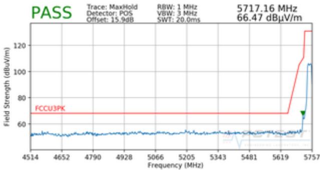
Plot 7-84. Radiated Lower Band Edge Plot (Peak – UNII Band 3)
