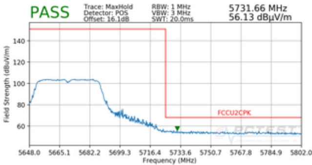
Plot 7-92. Radiated Upper Band Edge Plot (Peak – UNII Band 2C)
