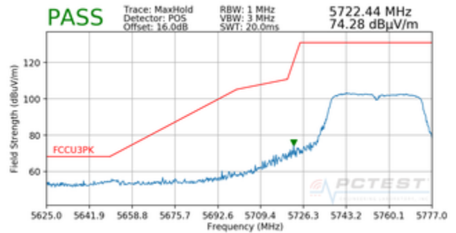
Plot 7-93. Radiated Lower Band Edge Plot (Peak – UNII Band 3)
