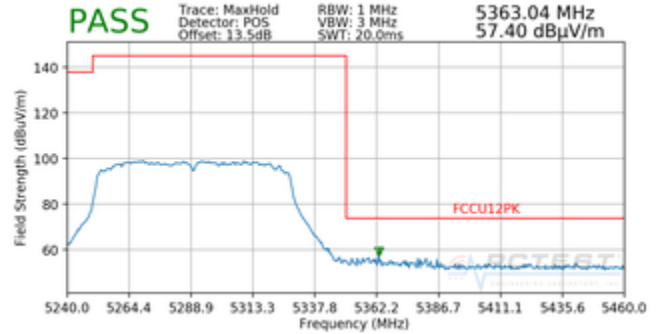
Plot 7-98. Radiated Upper Band Edge Plot (Peak – UNII Band 2A)
