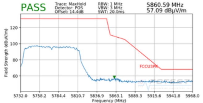
Plot 7-102. Radiated Upper Band Edge Plot (Peak – UNII Band 3)
