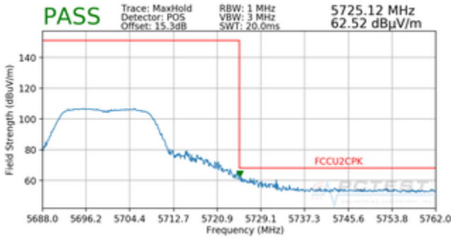
Plot 7-83. Radiated Upper Band Edge Plot (Peak – UNII Band 2C)
