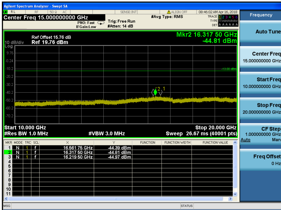
LTE Band 66 / 15MHz / QPSK - RB Size/Offset (1/74)–Low Channel
