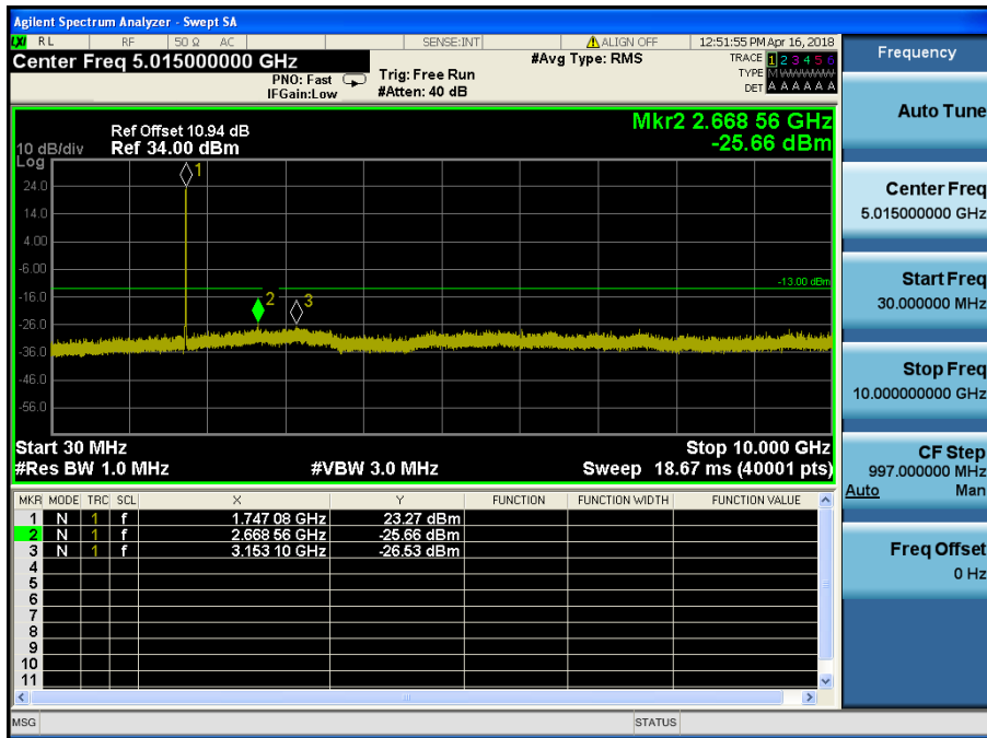
LTE Band 66 / 10MHz / 16QAM - RB Size/Offset (25/12) – Mid Channel
