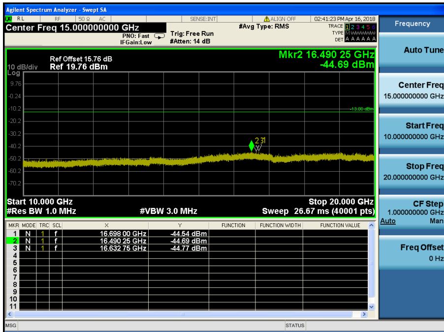
LTE Band 66 / 20MHz / 16QAM - RB Size/Offset (1/99) – High Channel
