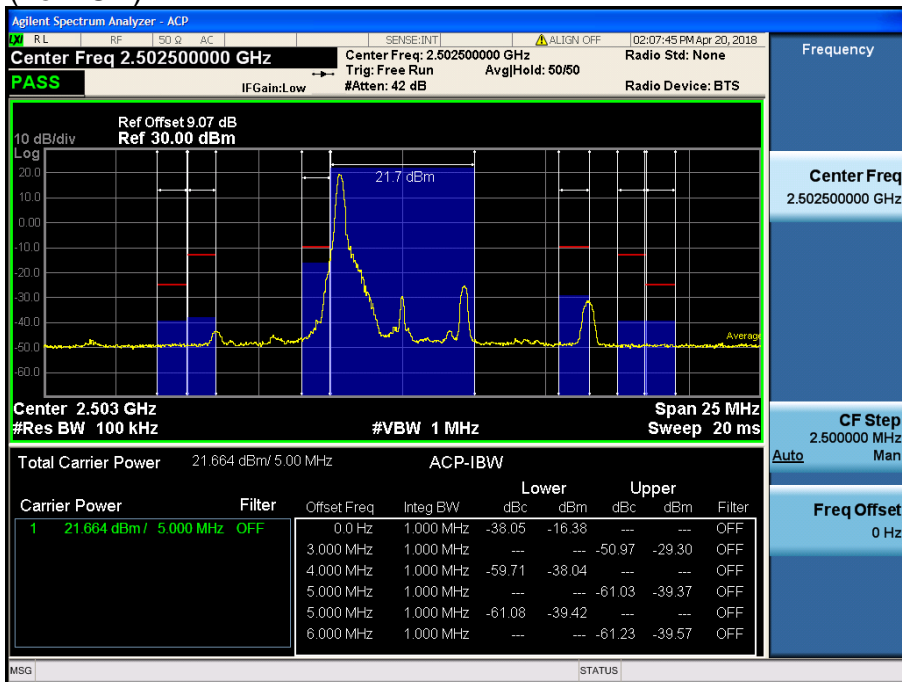
LTE Band 7 / 5MHz / QPSK - RB Size/Offset (1/0)
