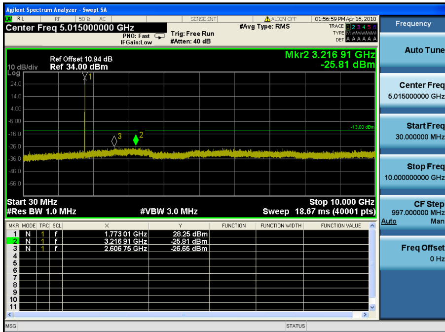
LTE Band 66 / 15MHz / 16QAM - RB Size/Offset (75/0) – High Channel
