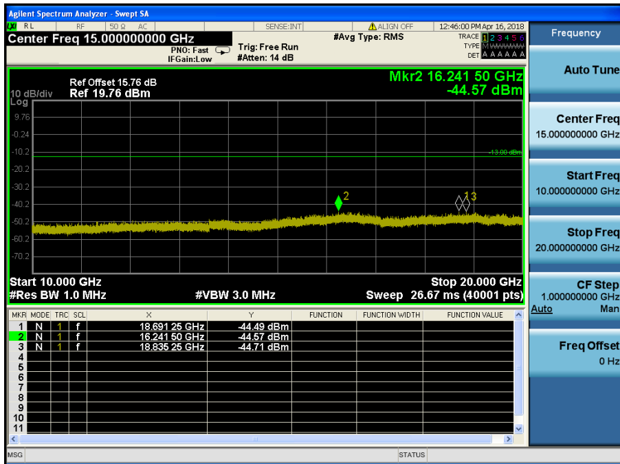
LTE Band 66 / 10MHz / 16QAM - RB Size/Offset (25/25) – Low Channel
