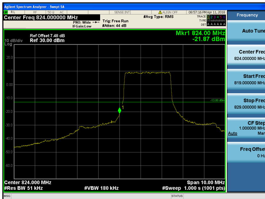
LTE Band 5 / 5MHz / QPSK Offset/Size (12/0)
