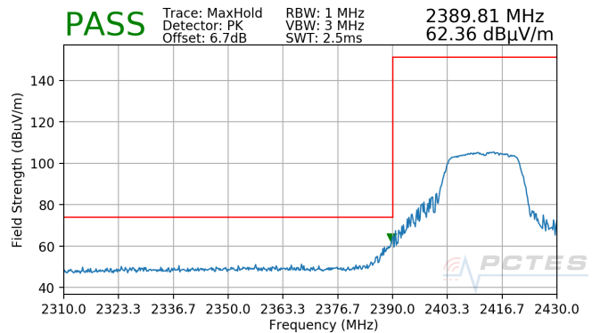
Plot 7-40. Radiated Restricted Lower Band Edge Measurement (Peak)
