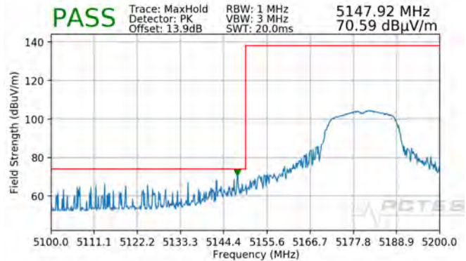
Plot 7-86. Radiated Lower Band Edge Plot (Peak – UNII Band 1)
