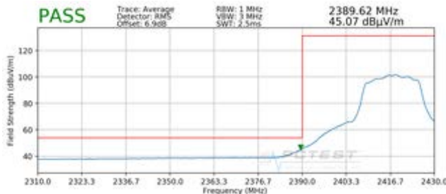
Plot 7-57. Radiated Restricted Lower Band Edge Measurement (Average)
