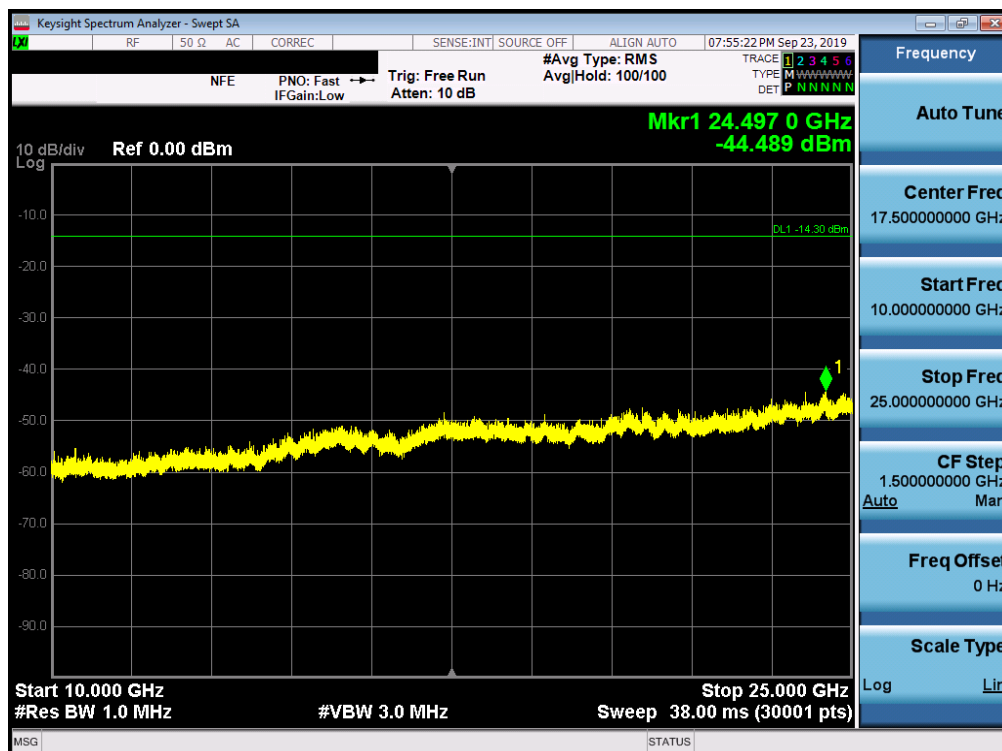
Plot 7-50. Conducted Spurious Plot (802.11ac – Ch. 11)
