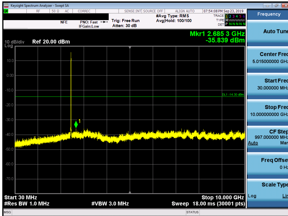
Plot 7-49. Conducted Spurious Plot (802.11ac – Ch. 11)
