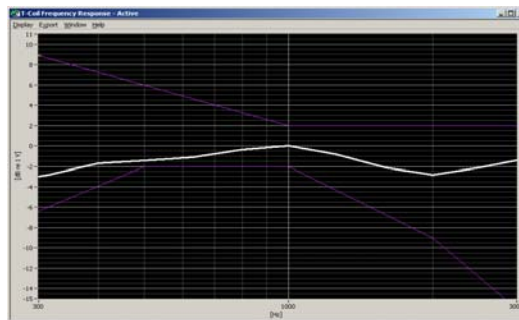
Figure 7-1 Axial Frequency Response
