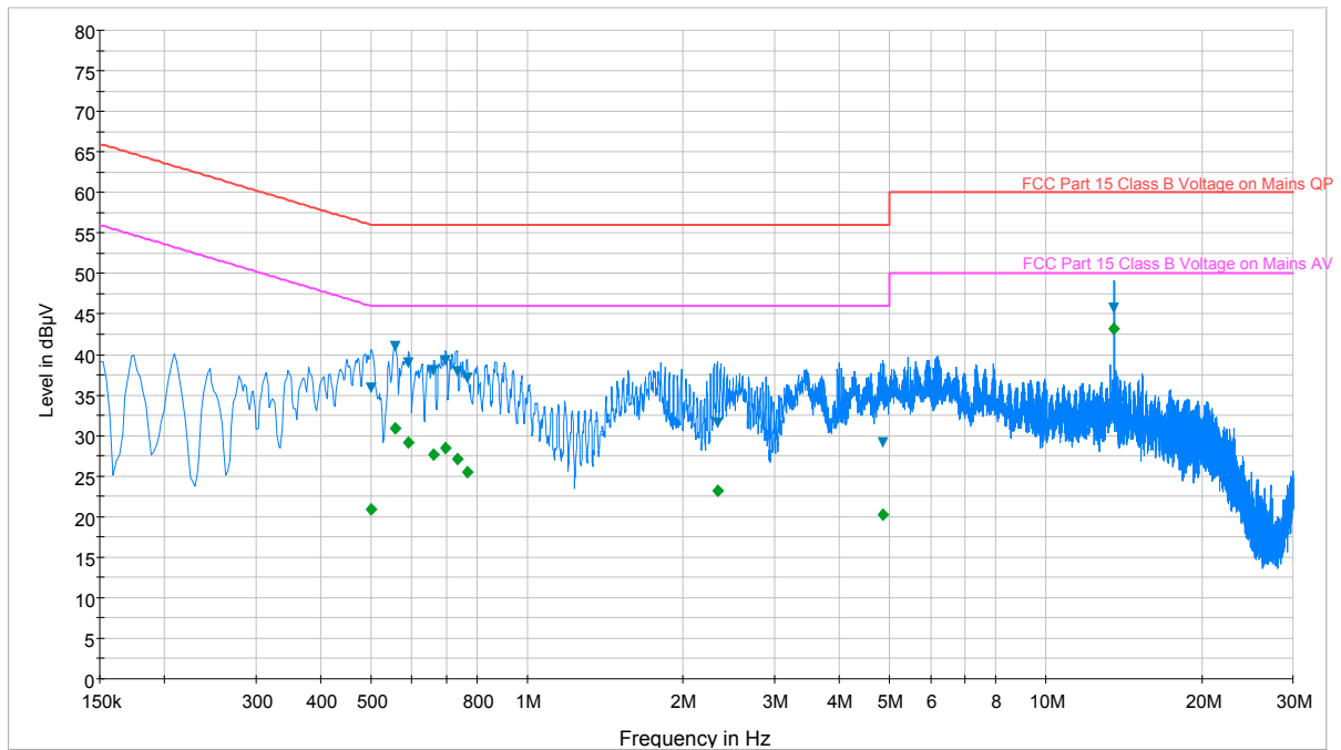
Plot 8-1. Line-Conducted Test Plot (L1)
