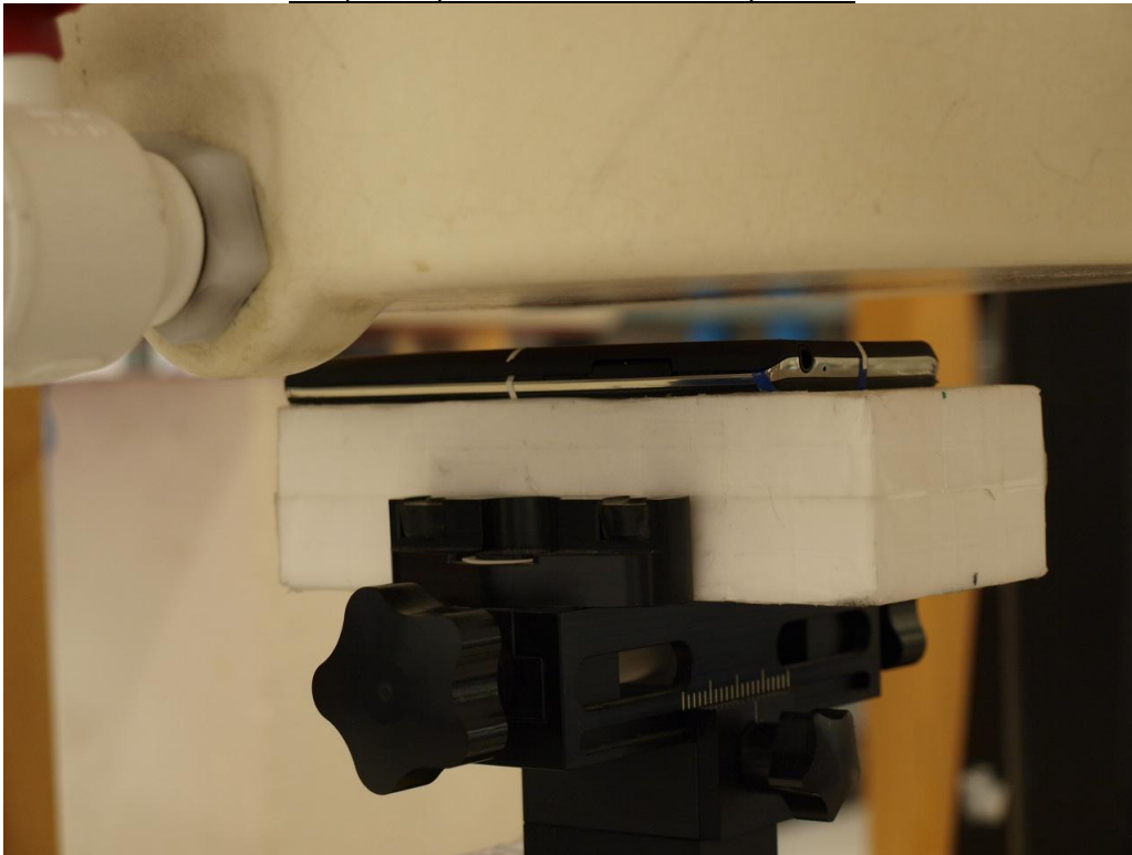
Body&Hotspo - Rear w/ 10 mm Separation (w/ Headset)
