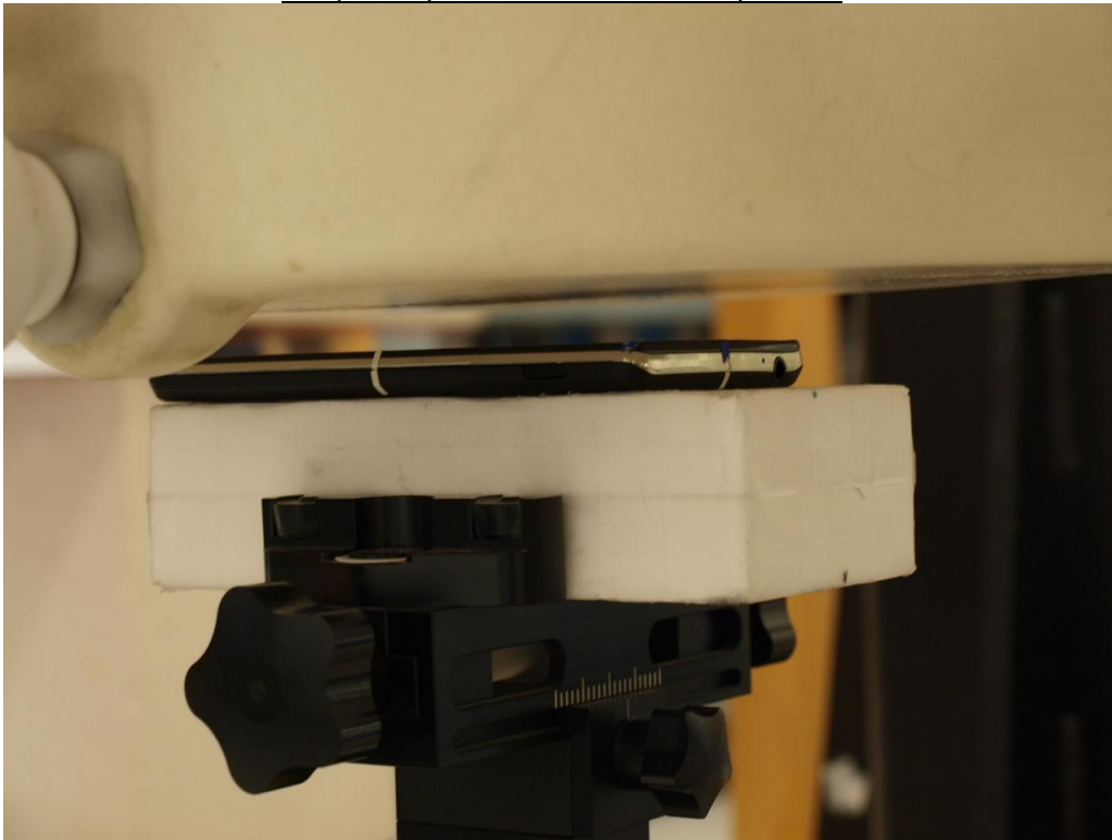
Body&Hotspot – Edge1 w/ 10 mm Separation
