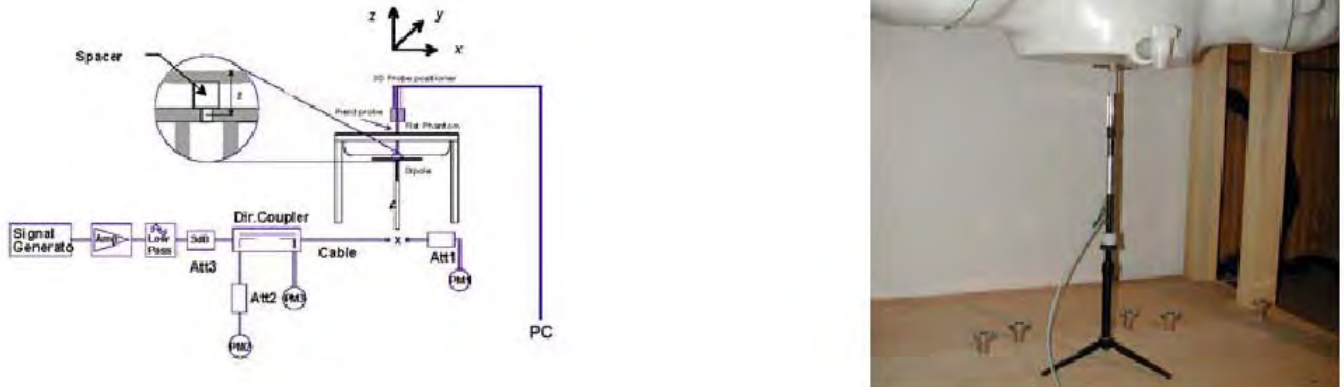
Figure 9.1 Dipole Validation Test Setup
